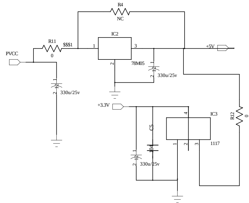
DC5V - DC3.3V
