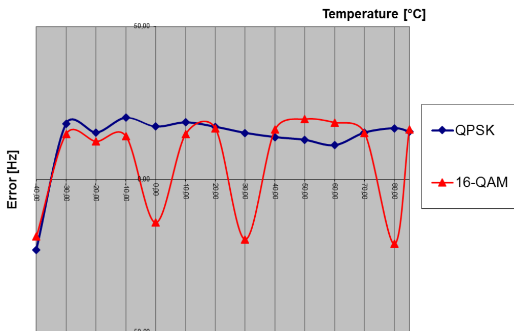
Frequency Error due to temperature variations LTE Band 4 / Channel High = 20375
