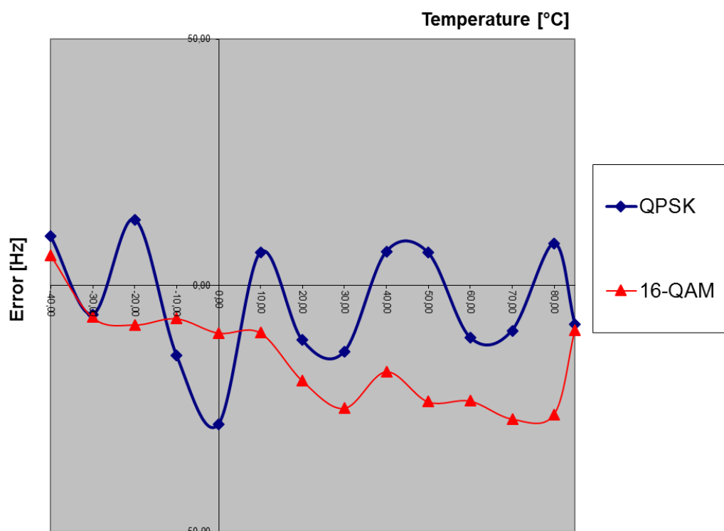
Frequency Error due to temperature variations LTE Band 13 / Channel Low = 23205
