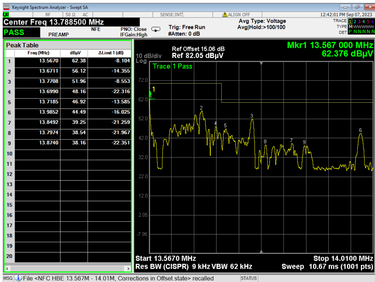
Figure 3 – Upper Bandedge
