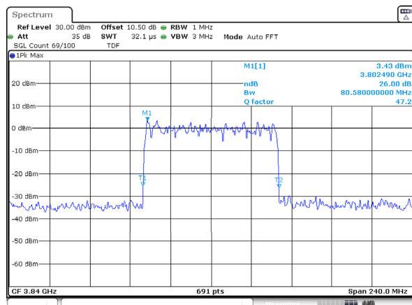
n77_3_80MHz_30kHz_3840MHz_CP-OFDM 16 QAM_RB217@0 26 dB Emission Bandwidth
