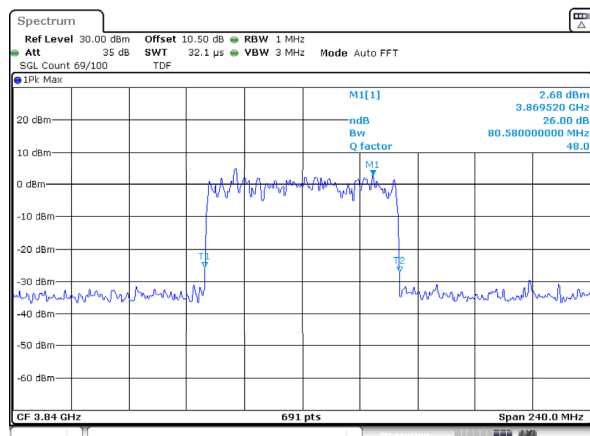
n77_3_80MHz_30kHz_3840MHz_CP-OFDM 64 QAM_RB217@0 26 dB Emission Bandwidth
