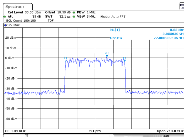
n77_3_80MHz_30kHz_3840MHz_CP-OFDM 256 QAM_RB217@0 Occupied Bandwidth
