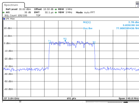
n77_3_80MHz_30kHz_3840MHz_CP-OFDM 64 QAM_RB217@0 Occupied Bandwidth
