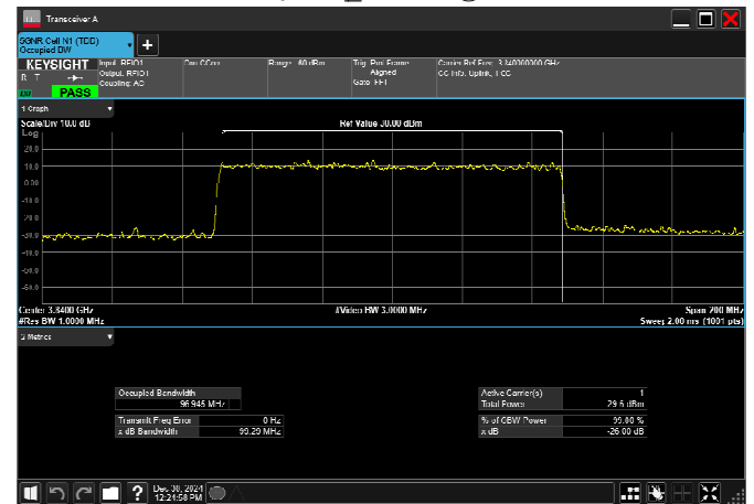
n77_3_100MHz_30kHz_3840MHz_DFT-s-OFDM 64 QAM_RB270@0
