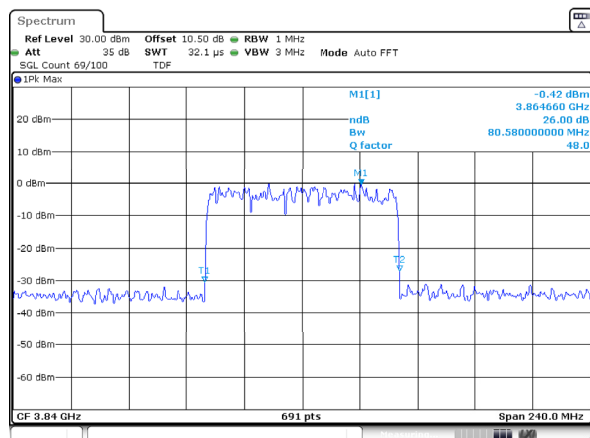
n77_3_80MHz_30kHz_3840MHz_CP-OFDM 256 QAM_RB217@0 26 dB Emission Bandwidth
