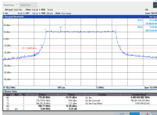
Band13-5MHz-QPSK-23230-25RB#0
