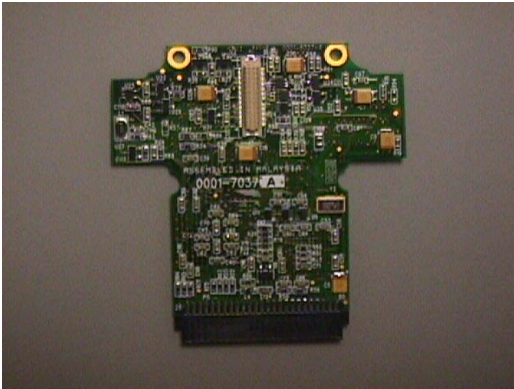
Micro Tri-Reader® Digital Board Side 1
