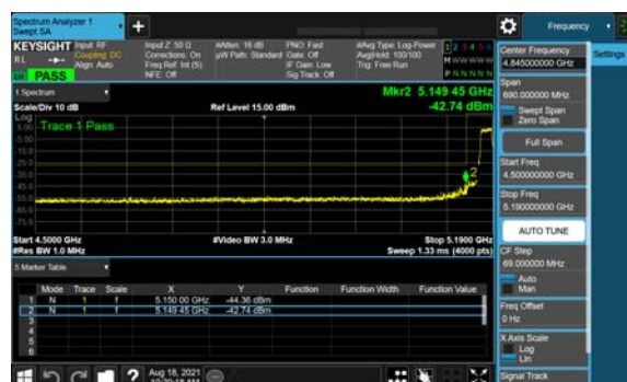
Antenna B
