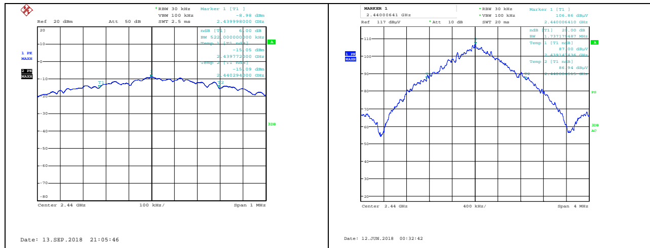
2MBit/s, Channel 19 (2440MHz) 6dB BW (left) 20dB BW(right)
