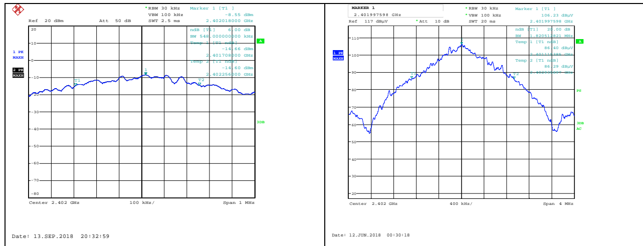
2MBit/s, Channel 0 (2402MHz) 6dB BW (left) 20dB BW(right)
