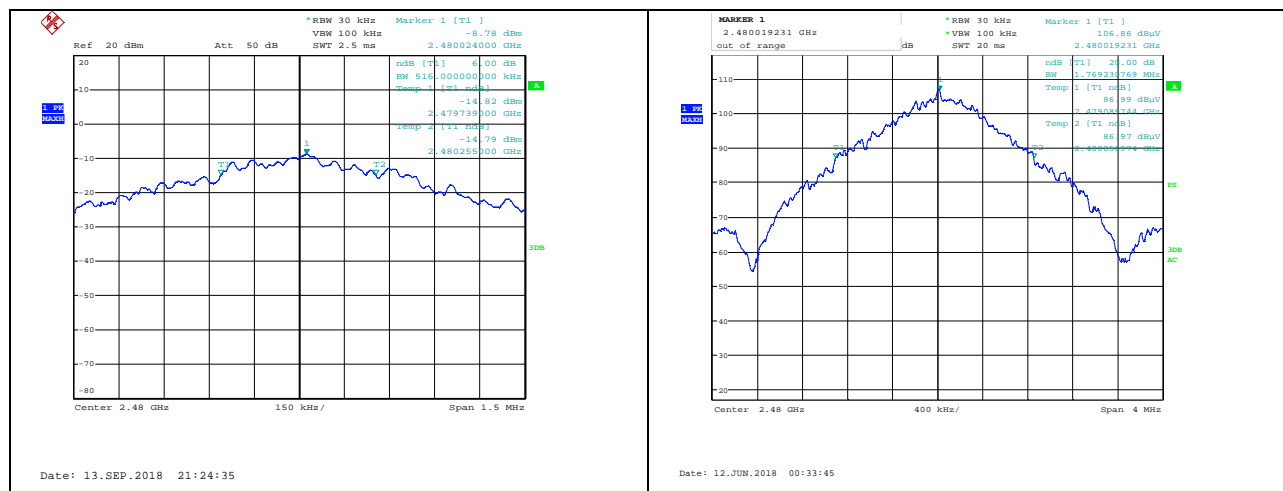
2MBit/s, Channel 39 (2480MHz) 6dB BW (left) 20dB BW(right)
