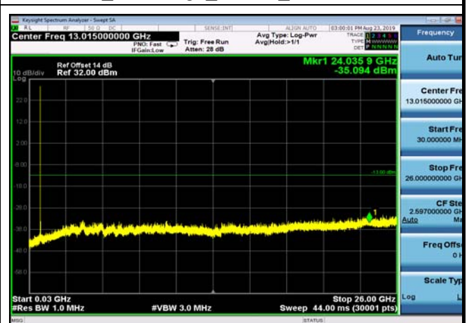
FDD05_LowRange_10MHz_30MHz~26GHz
