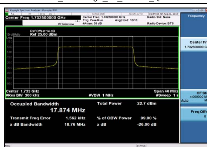
FDD04_MidRange_20_1732.5_QPSK
