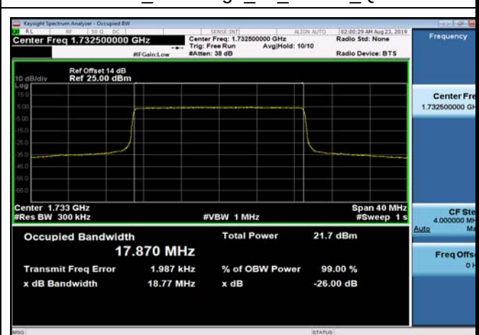
FDD04_MidRange_20_1732.5_Q16
