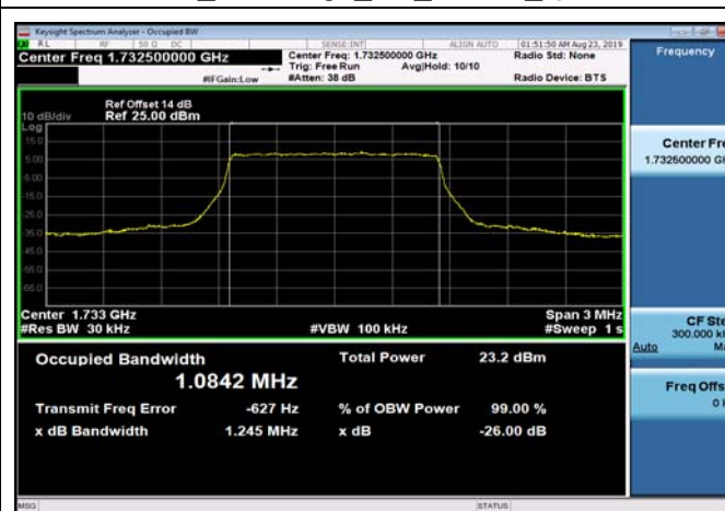
FDD04_MidRange_3_1732.5_QPSK
