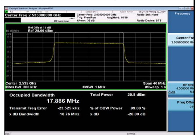
FDD07_MidRange_20MHz_2535MHz_Q16
