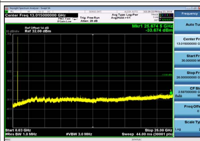
FDD05_LowRange_1.4MHz_30MHz~26GHz
