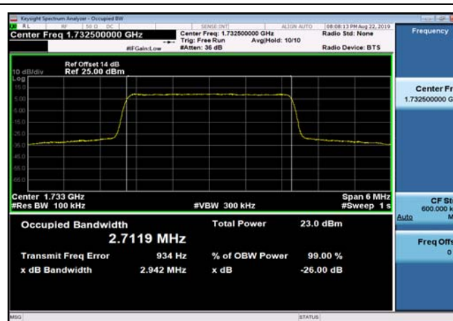
FDD04_MidRange_3MHz_1732.5MHz_QPSK
