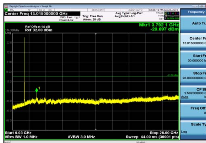
FDD02_HighRange_3MHz_30MHz~26GHz
