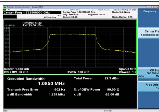
FDD04_MidRange_3_1732.5_Q16
