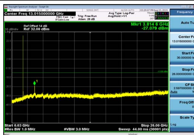
FDD02_HighRange_3MHz_30MHz~26GHz
