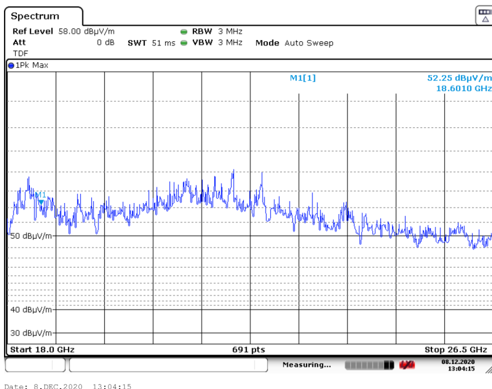
Plot 9: Pre-scan plot with peak detector. Radiated emissions from 18 GHz – 26.5 GHz, 5GHz + BT mode
