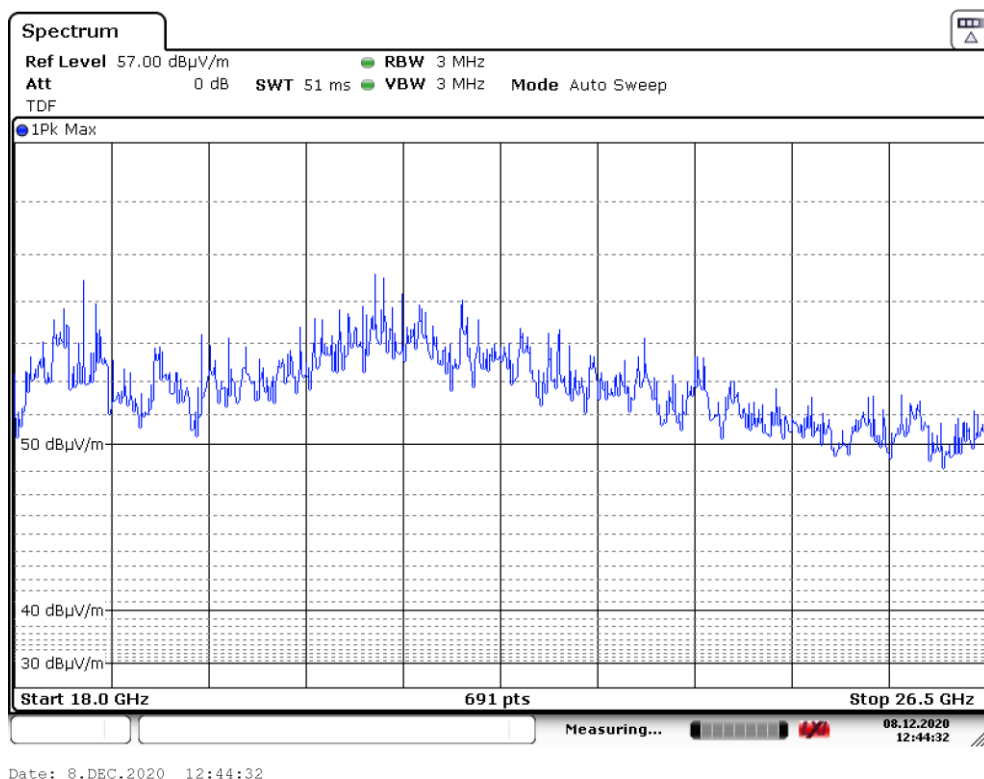
Plot 10: Pre-scan plot with peak detector. Radiated emissions from 18 GHz – 26.5 GHz, 2.4GHz mode
