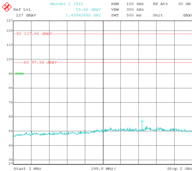
Title: ATWILC3000 Comment A: Conducted Spurious Bluetooth 2402 MHz Date: 23.SEP.2015 13:39:46
