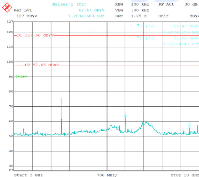
Title: ATWILC3000 Comment A: Conducted Spurious Bluetooth 2402 MHz Date: 23.SEP.2015 13:41:30
