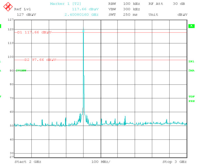
Title: ATWILC3000 Comment A: Conducted Spurious Bluetooth 2402 MHz Date: 23.SEP.2015 13:39:11
