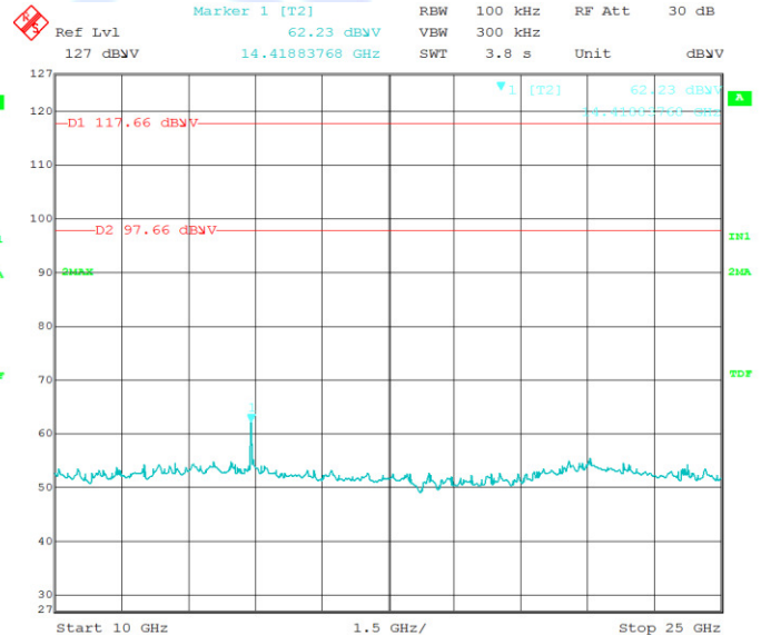
Title: ATWILC3000 Comment A: Conducted Spurious Bluetooth 2402 MHz Date: 23.SEP.2015 13:42:55
