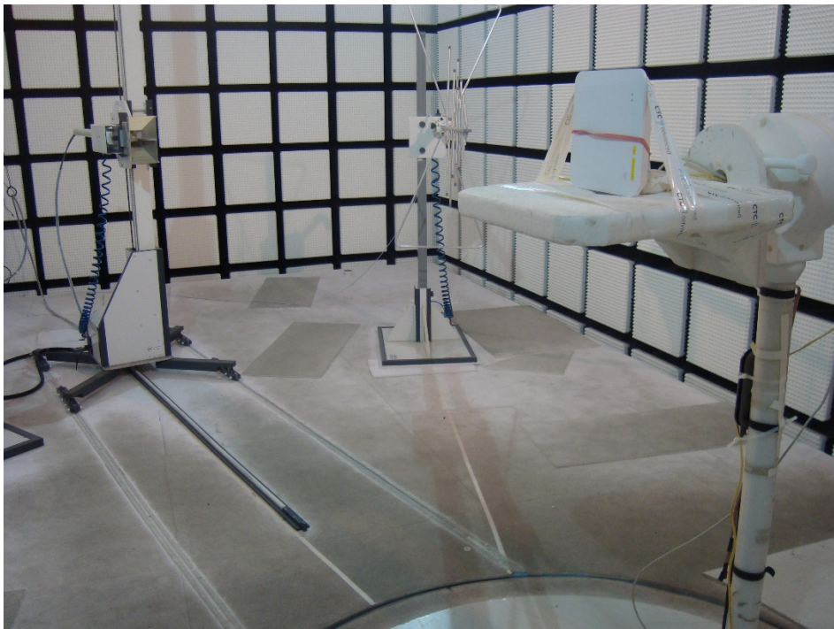
Photo 2: Radiated Emission
