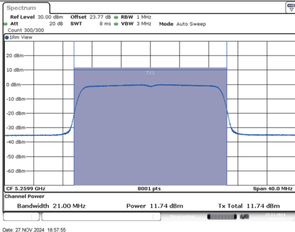
11AX20MIMO-Ant2-5260-PASS
