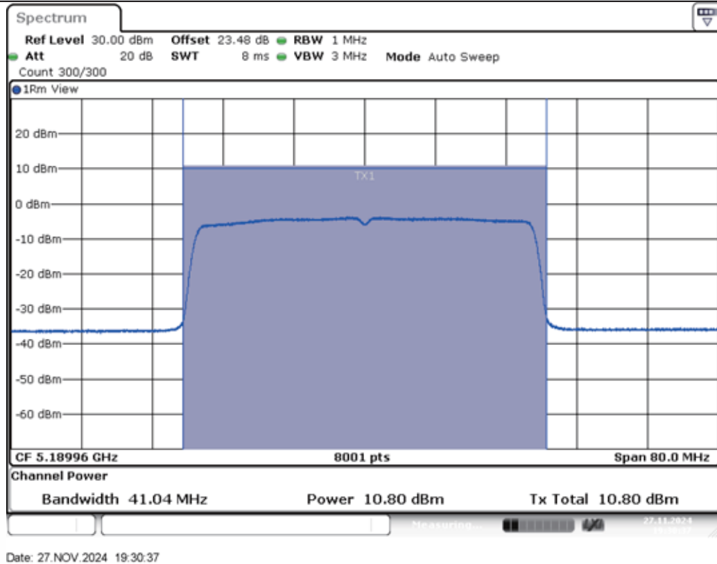
11AX40MIMO-Ant2-5190-PASS
