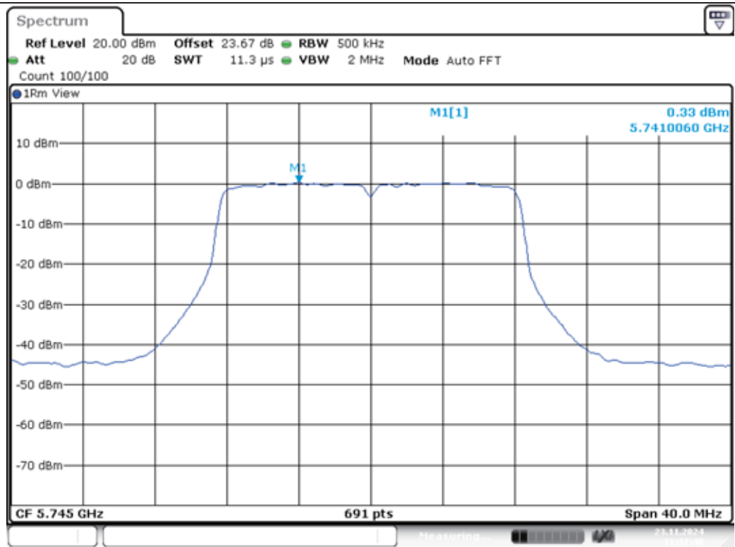
11A-Ant1-5745-PASS
