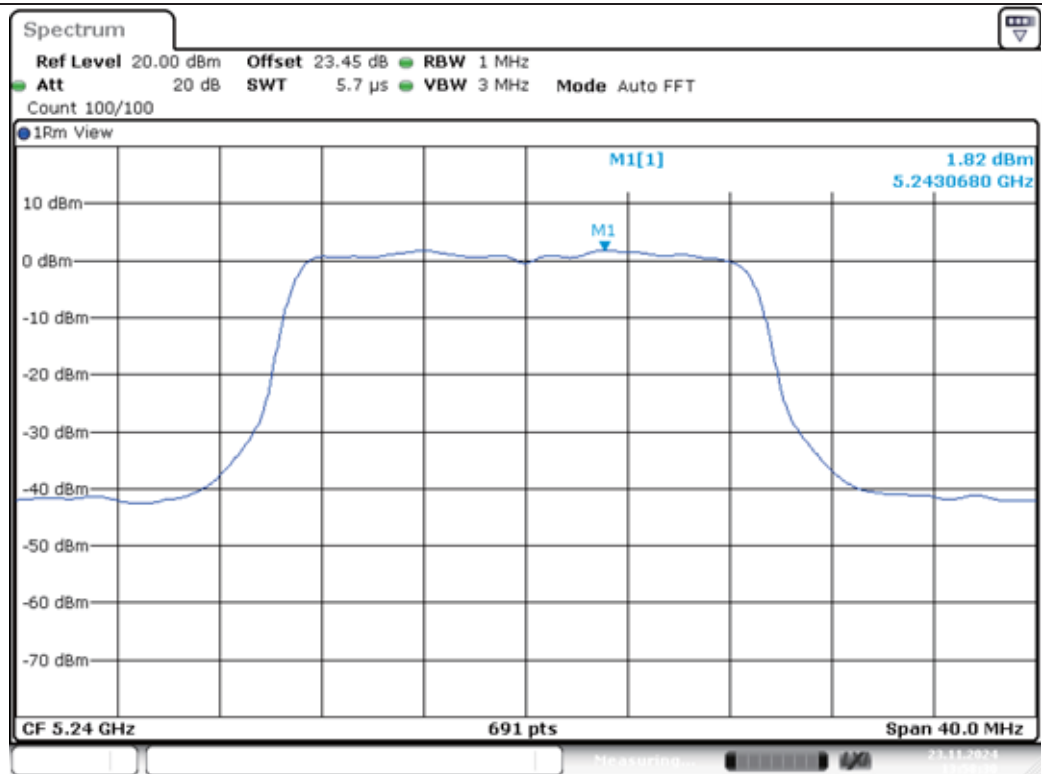
11N20MIMO-Ant1-5240-PASS
