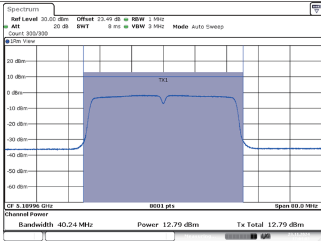
11AC40MIMO-Ant1-5190-PASS
