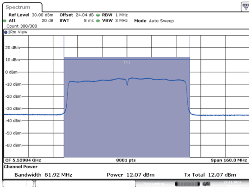
11AC80MIMO-Ant1-5530-PASS
