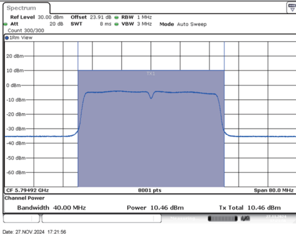
11AC40MIMO-Ant2-5795-PASS
