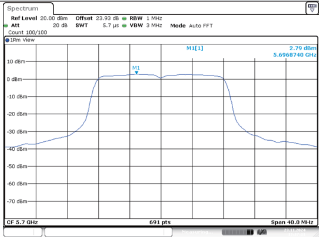
11A-Ant1-5700-PASS
