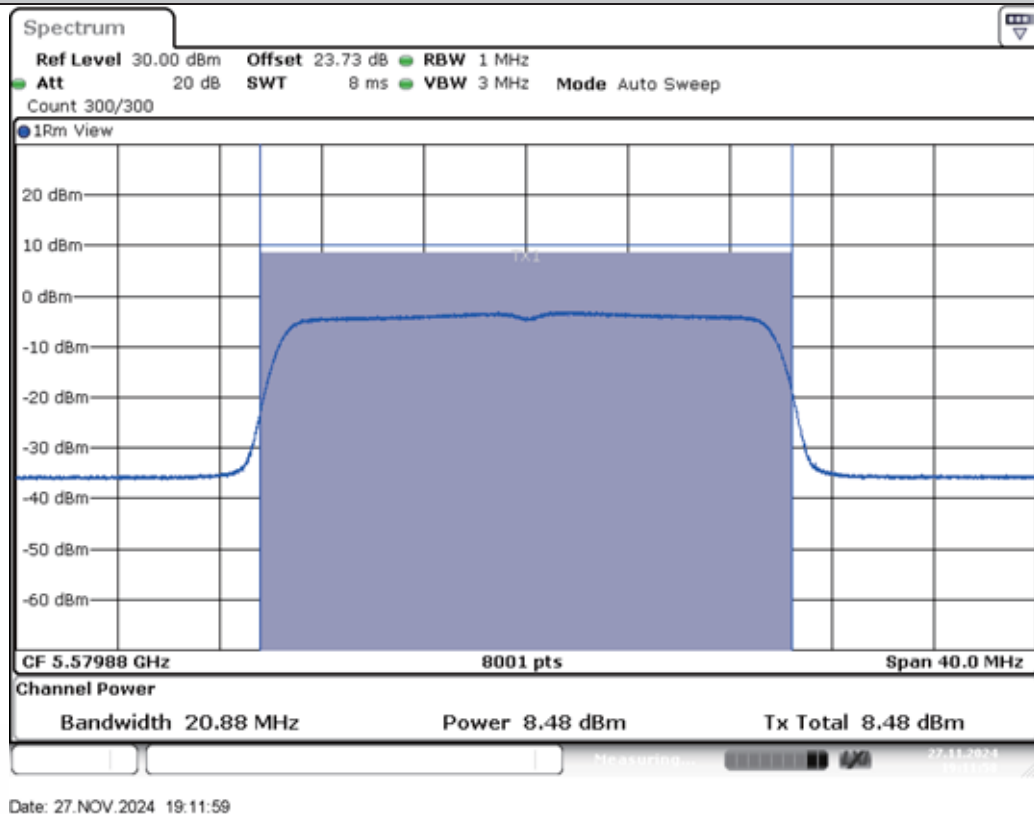
11AX20MIMO-Ant2-5580-PASS
