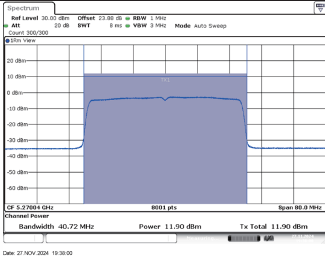
11AX40MIMO-Ant2-5270-PASS
