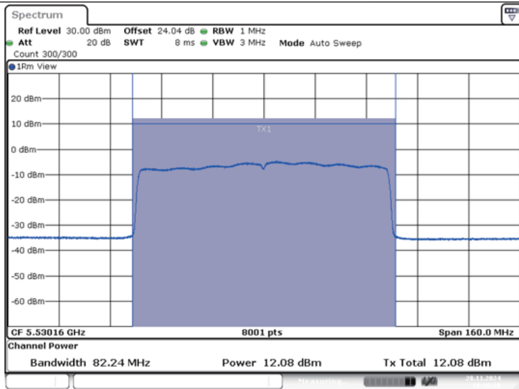
11AX80MIMO-Ant1-5530-PASS
