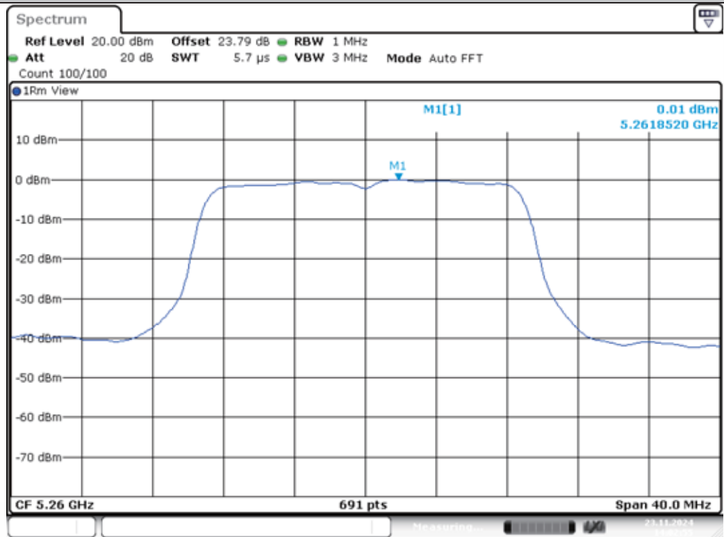
11N20MIMO-Ant1-5260-PASS
