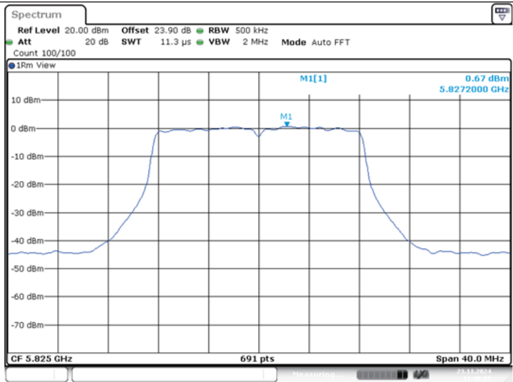
11A-Ant1-5825-PASS
