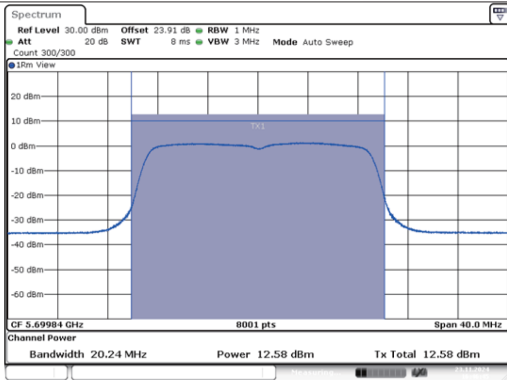
11AC20MIMO-Ant1-5700-PASS
