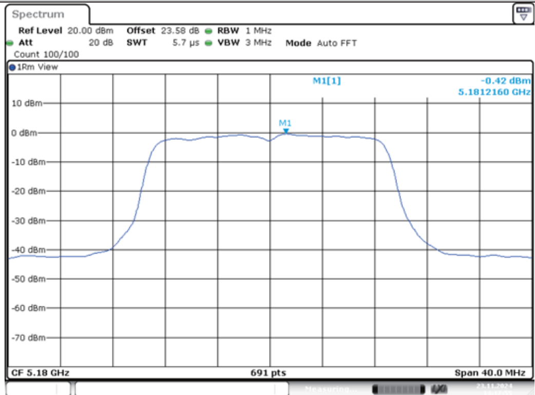
11N20MIMO-Ant1-5180-PASS
