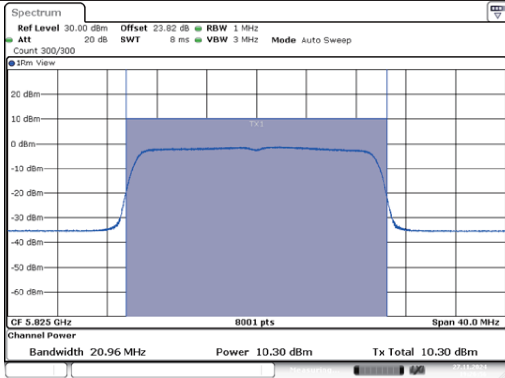
11AX20MIMO-Ant1-5825-PASS
