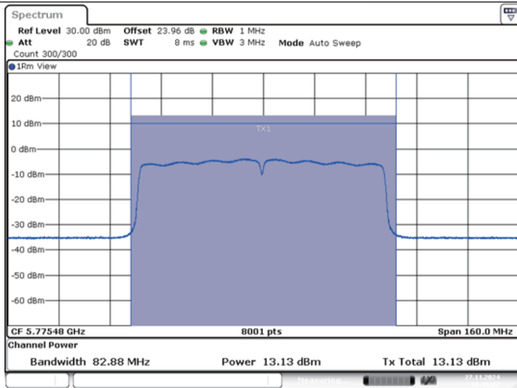
11AC80MIMO-Ant1-5775-PASS
