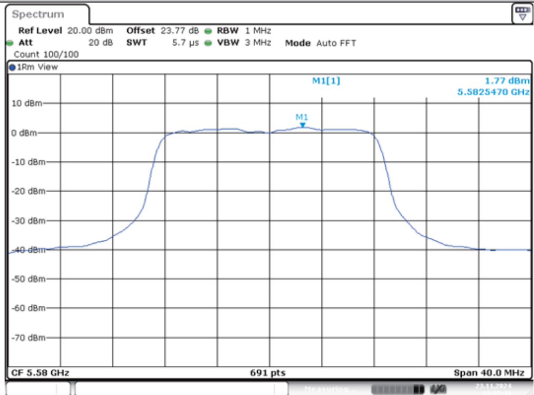
11A-Ant1-5580-PASS
