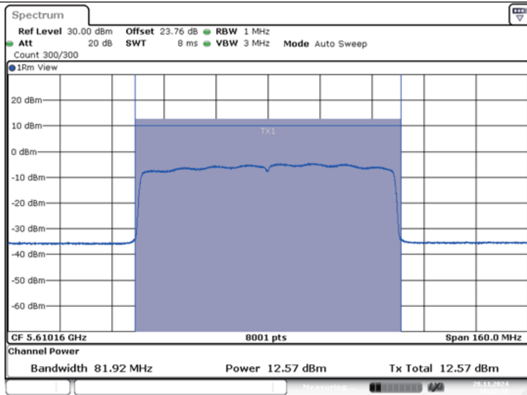
11AX80MIMO-Ant1-5610-PASS
