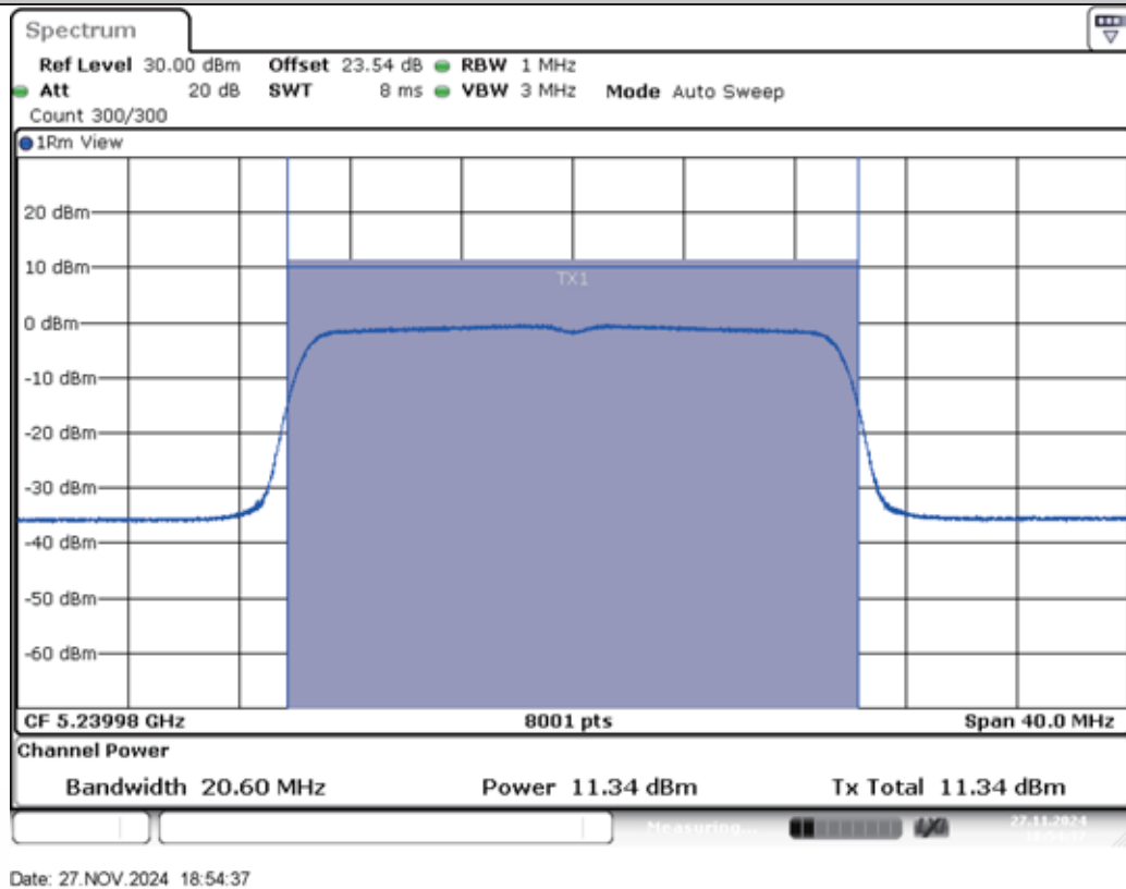
11AX20MIMO-Ant2-5240-PASS
