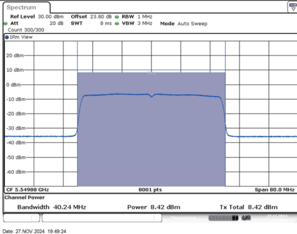
11AX40MIMO-Ant2-5550-PASS
