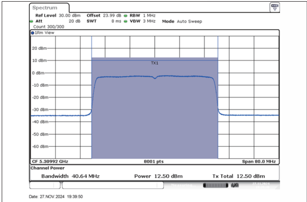
11AX40MIMO-Ant1-5310-PASS
