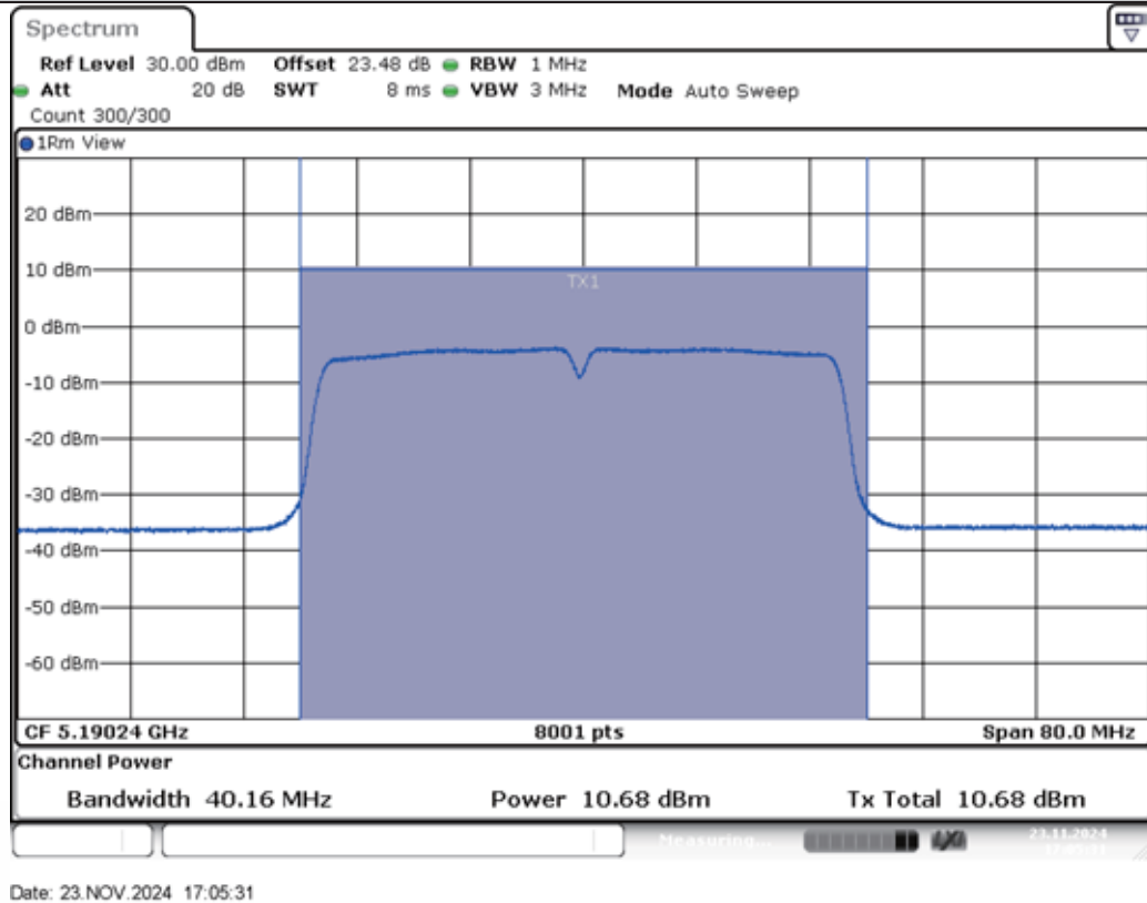
11AC40MIMO-Ant2-5190-PASS
