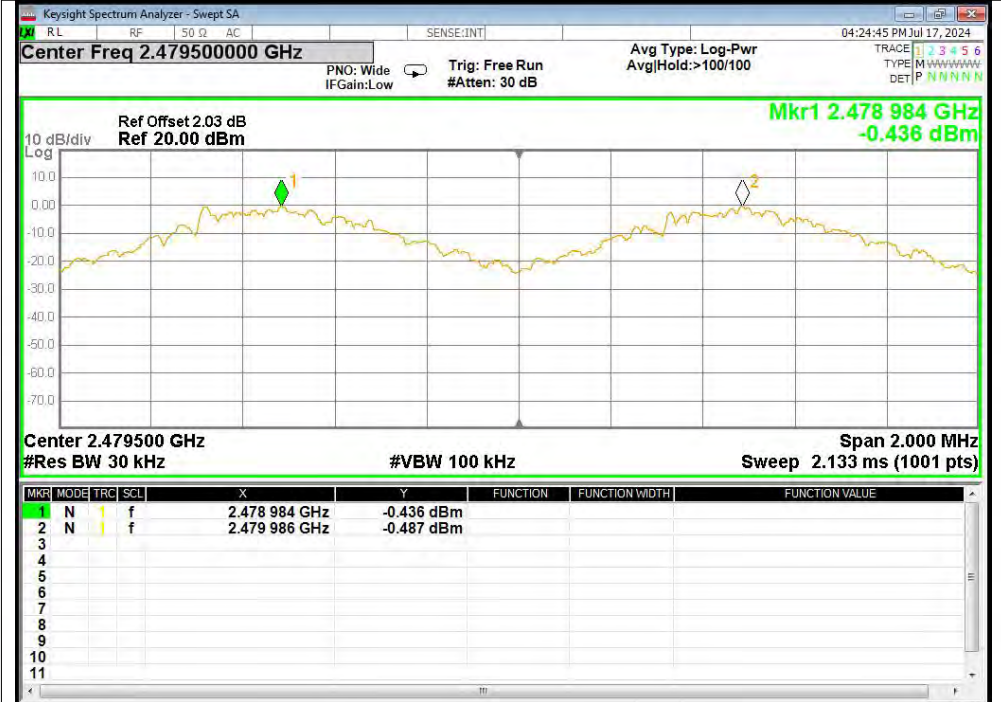
CFS NVNT 2-DH5 2480MHz Ant1
