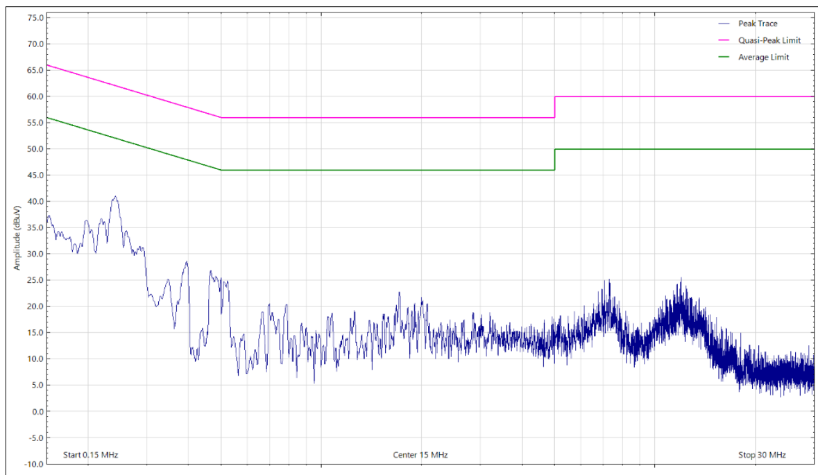
Figure 12 - Live Line - 150 kHz to 30 MHz
