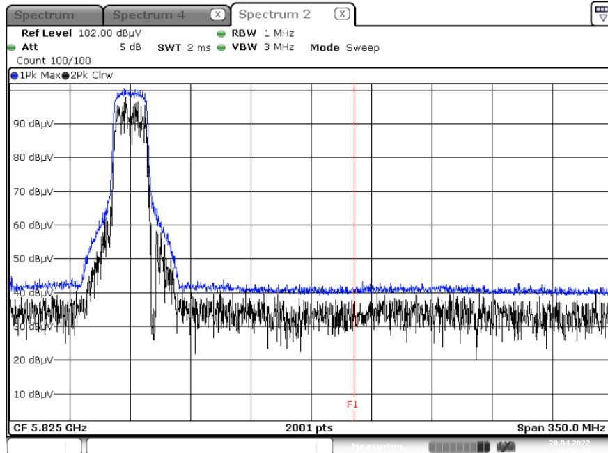
Peak result (802.11ax(HE20), Ch.144, SU, Y-V)
