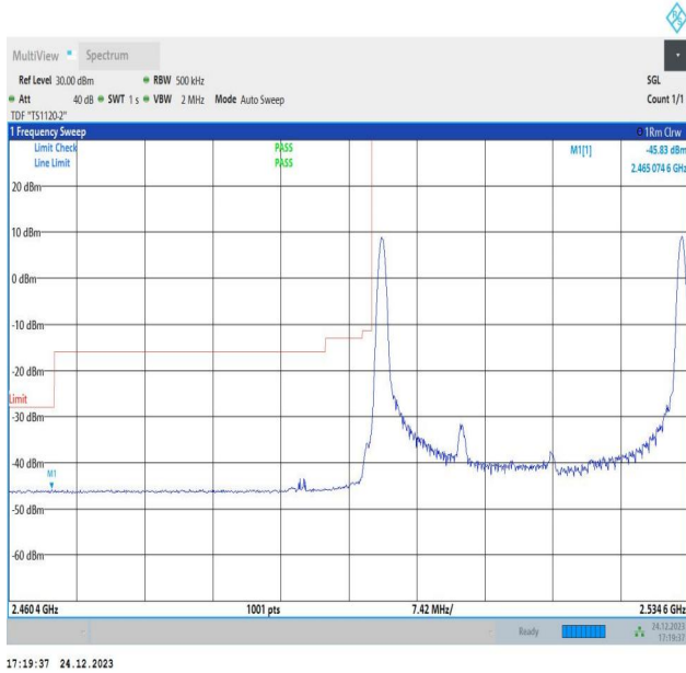
20MHz-15MHz_16QAM@16QAM-16QAM@16QAM_20850-21021_1RB#0@100RB#0-1RB#74@75RB#0
