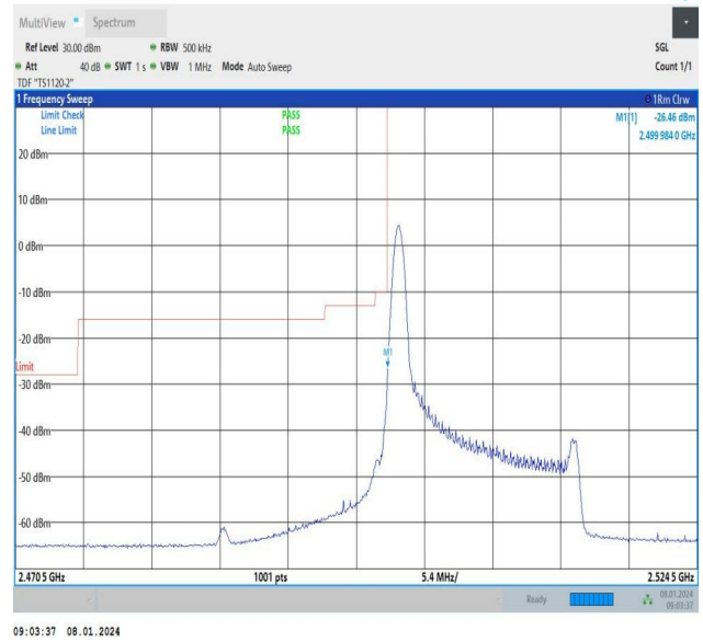
15MHz-10MHz_64QAM@64QAM-64QAM_20825-2 0945_1RB#0@75RB#0-0RB#0@50RB#0
