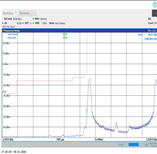
15MHz-10MHz_64QAM@64QAM-64QAM@64QAM_20825-20945_1RB#0@75RB#0-1RB#49@49RB#0
