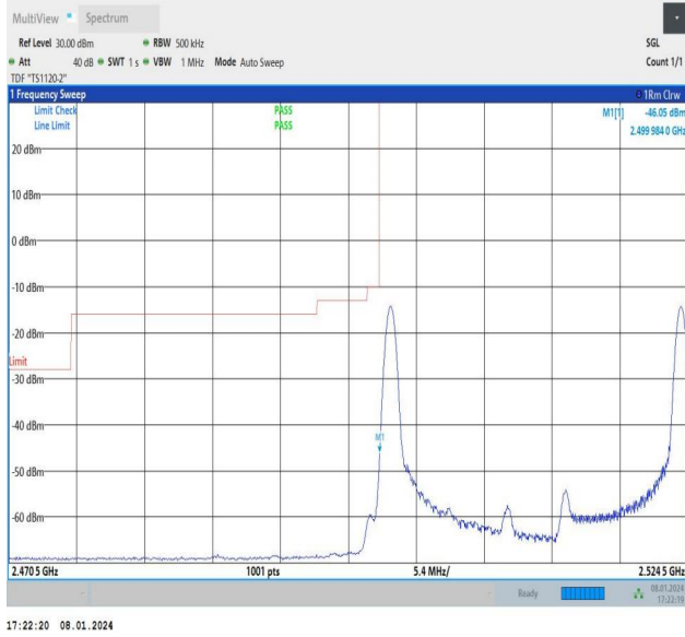
15MHz-10MHz_QPSK@QPSK-QPSK@QPSK_20825-20945_1 RB#0@75RB#0-1RB#49@49RB#0
