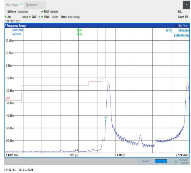
15MHz-10MHz_16QAM@16QAM-16QAM@16QAM_20825-20945_1RB#0@75RB#0-1RB#49@49RB#0
