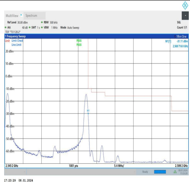
15MHz-10MHz_QPSK@QPSK-QPSK@QPSK_21277-21397_1RB#0@75RB#0-1RB#49@49RB#0
