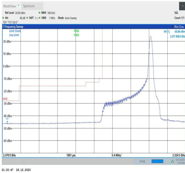
15MHz-10MHz_64QAM@64QAM-64QAM_20825-20 945_1RB#74@75RB#0-0RB#0@50RB#0
