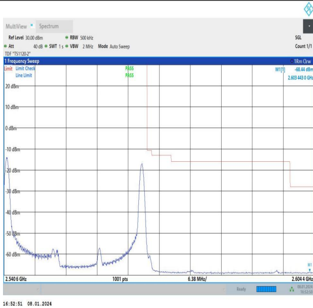
10MHz-20MHz_64QAM@64QAM-64QAM_21206-21 350_1RB#0@50RB#0-1RB#99@100RB#0
