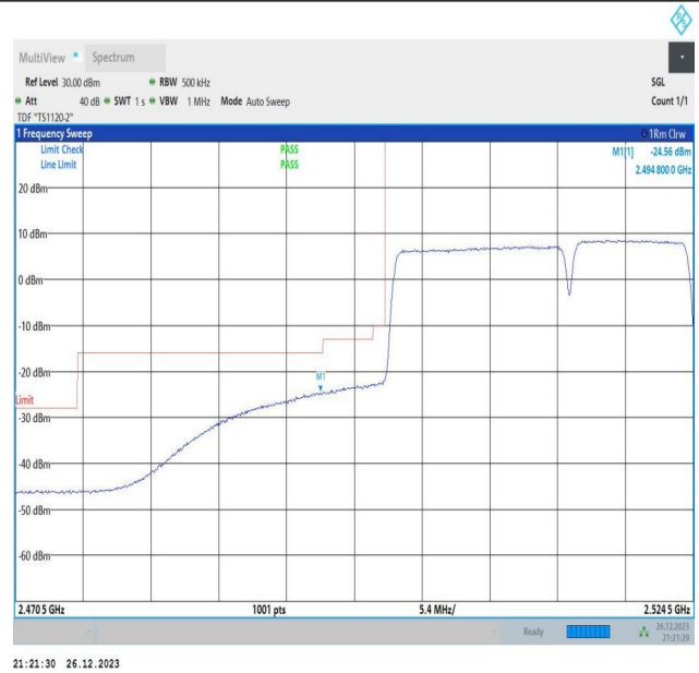
15MHz-10MHz_64QAM@64QAM-64QAM_20825-2 0945_75RB#0@75RB#0-50RB#0@50RB#0
