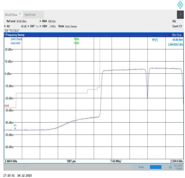
20MHz-15MHz_QPSK@QPSK-QPSK@QPSK_20850-21021_100RB#0@100RB#0-75RB#0@75RB#0
