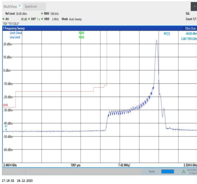
20MHz-15MHz_16QAM@16QAM-16QAM@16QAM_20850-21021_1RB#99@100RB#0-0RB#0@75RB#0
