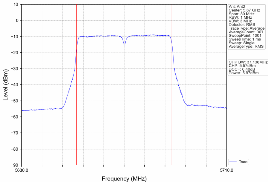
802.11ac(VHT40)_HCH_5670MHz_Ant2_NTNV
