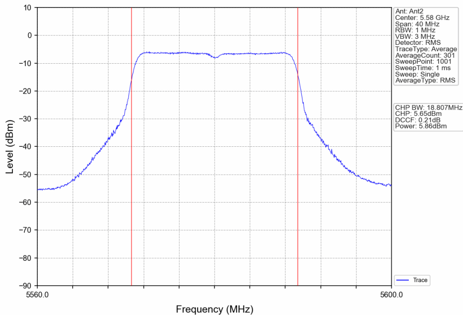
802.11ac(VHT20)_MCH_5580MHz_Ant2_NTNV
