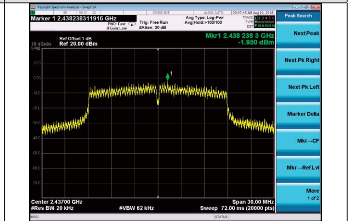
11nHT20-MCH
