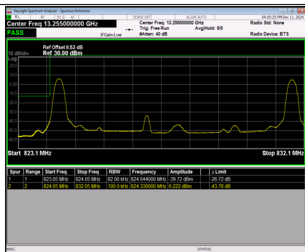
5-5-3MHz-5MHz-16QAM@16QAM-16QAM-2041
