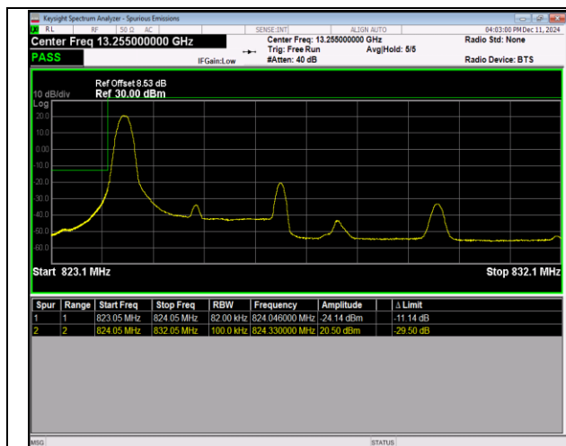
5-5-3MHz-5MHz-QPSK@QPSK-QPSK-20416-20 455-1RB#0@15RB#0-0RB#0@25RB#0-PASS
