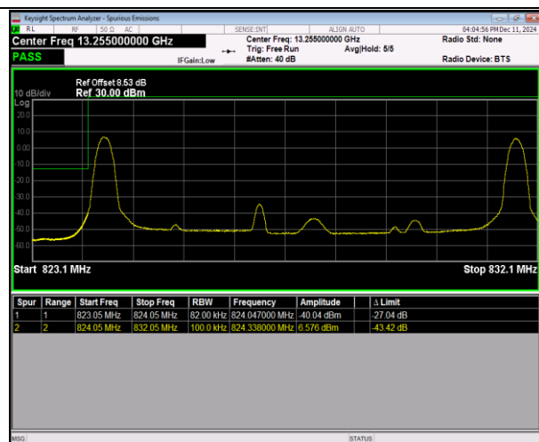
5-5-3MHz-5MHz-QPSK@QPSK-QPSK-20416-204 55-1RB#0@15RB#0-1RB#24@25RB#0-PASS
