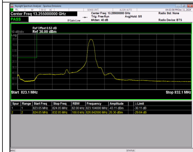
5-5-3MHz-5MHz-QPSK@QPSK-QPSK-20416-20 455-1RB#14@15RB#0-0RB#0@25RB#0-PASS
