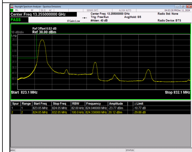
5-5-3MHz-5MHz-16QAM@16QAM-16QAM-204
