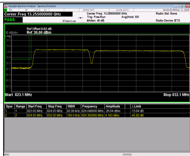
5-5-3MHz-5MHz-QPSK@QPSK-QPSK-20416-204 55-15RB#0@15RB#0-25RB#0@25RB#0-PASS
