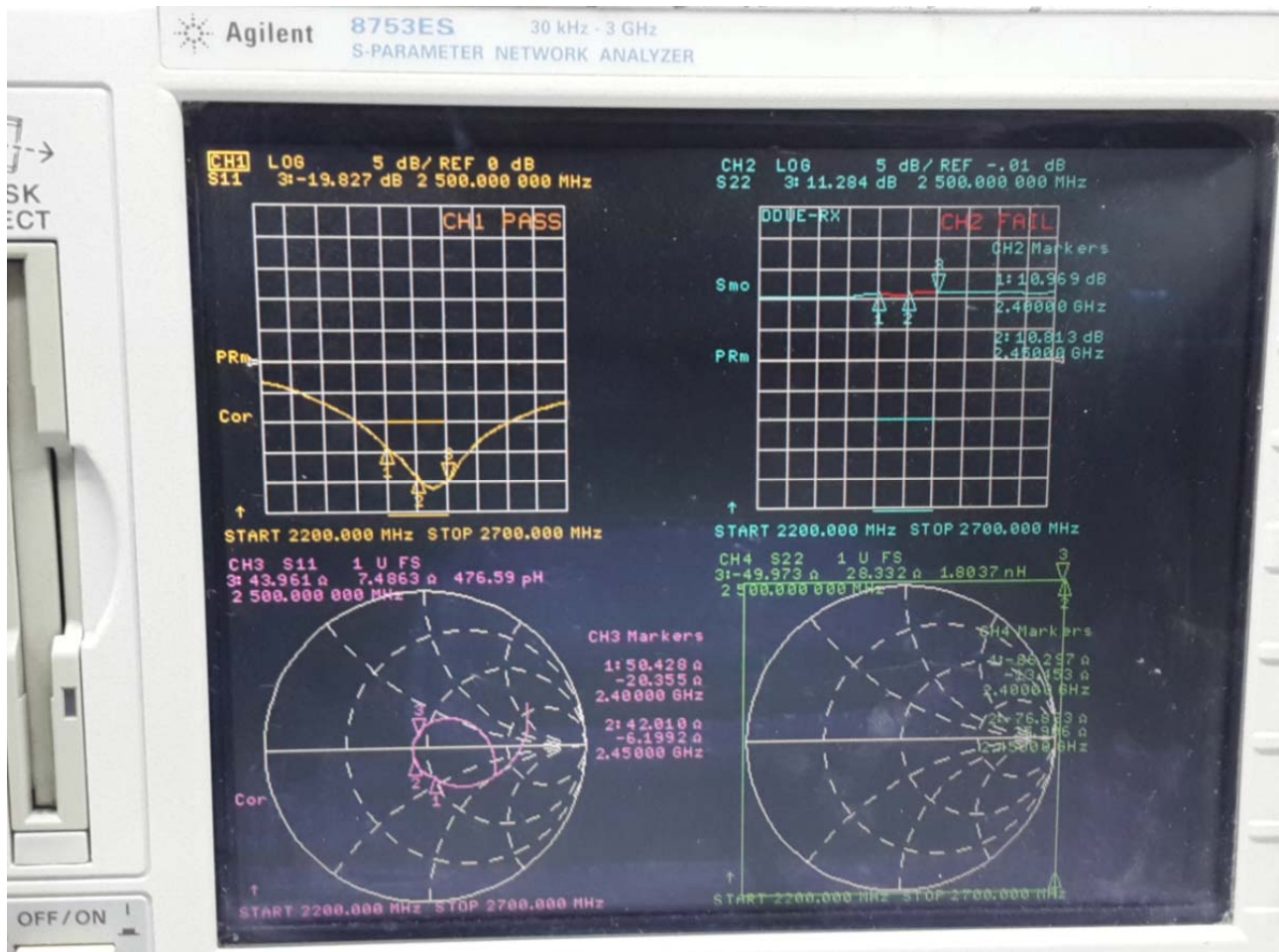
RF Antenna Assembly SPEC:2.4~2.5GHz
