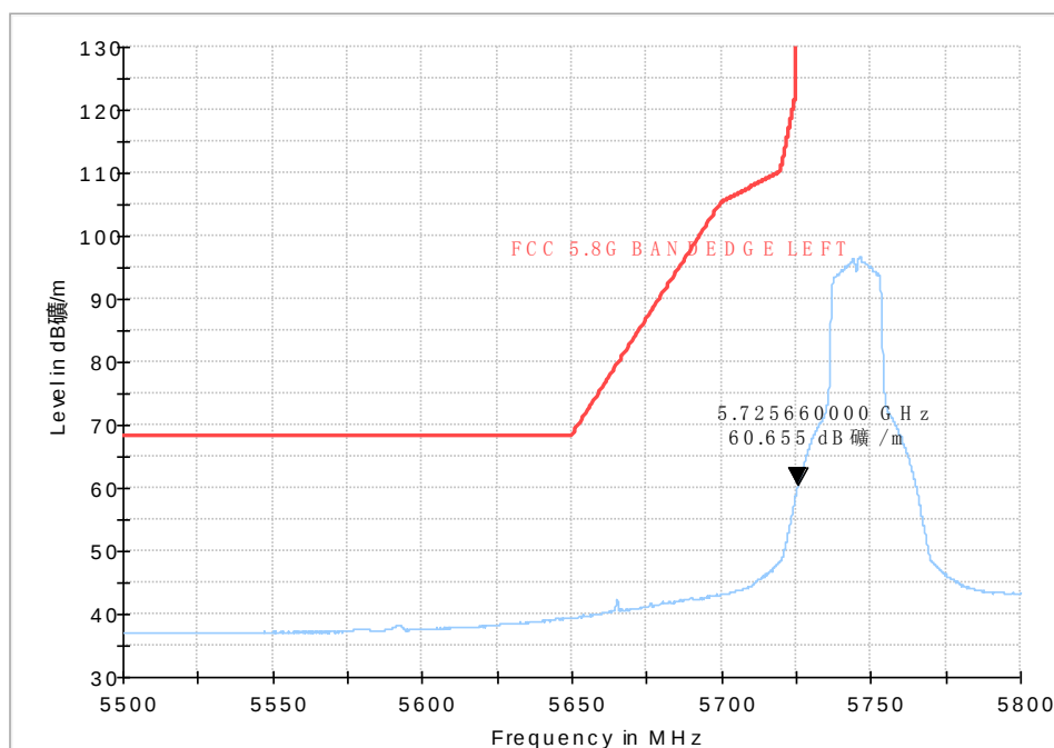
Fig. 47 Band Edges (802.11a, 5745MHz)
