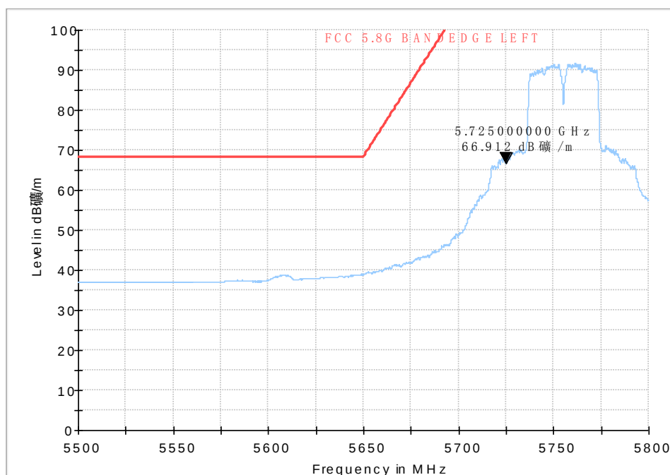
Fig. 51 Band Edges (802.11n-HT40, 5755MHz)
