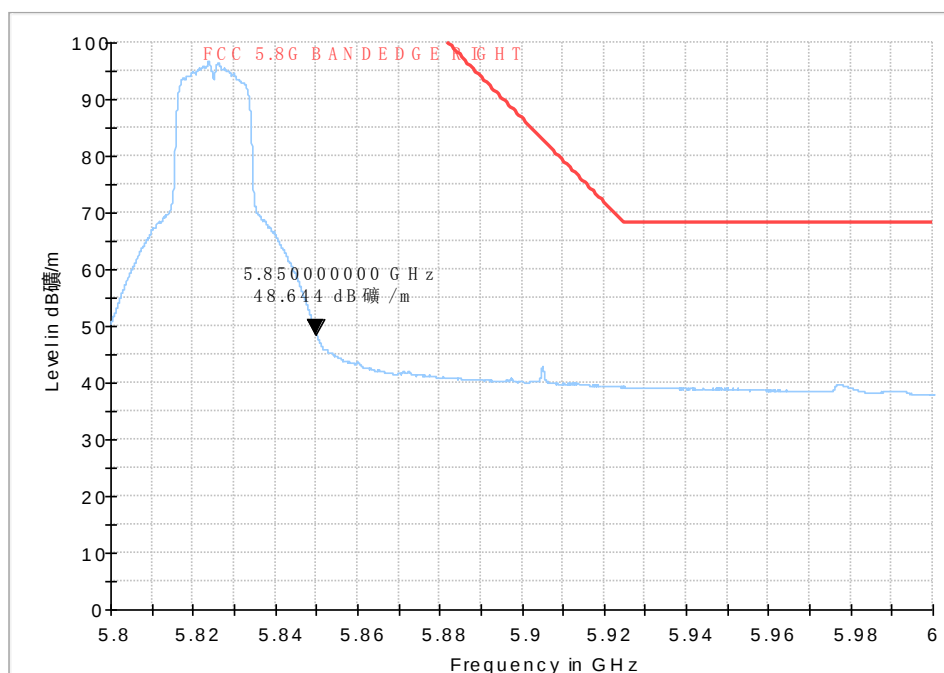
Fig. 50 Band Edges (802.11n-HT20, 5825MHz)
