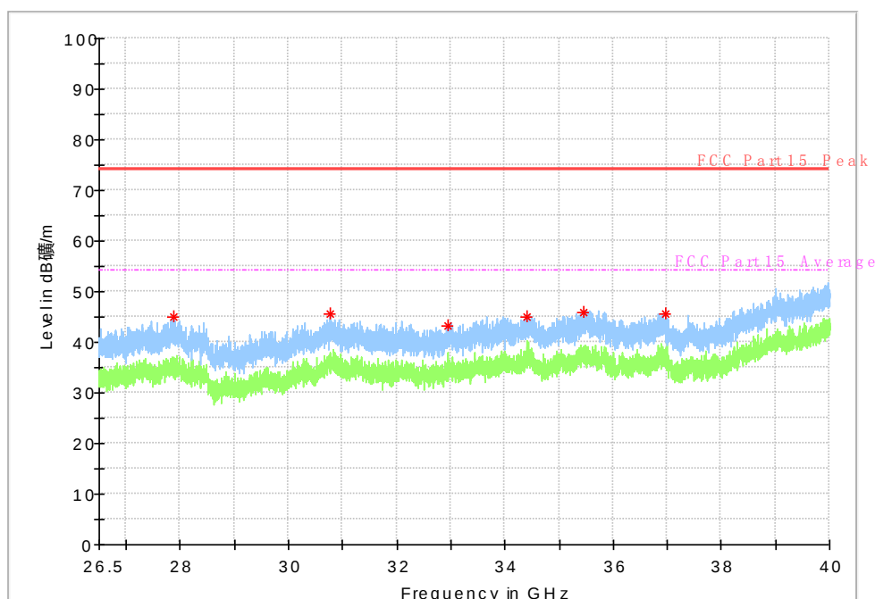
Fig. 46 Radiated emission: 802.11n, (802.11n-HT40, Ch151, 26.5 GHz - 40 GHz)
