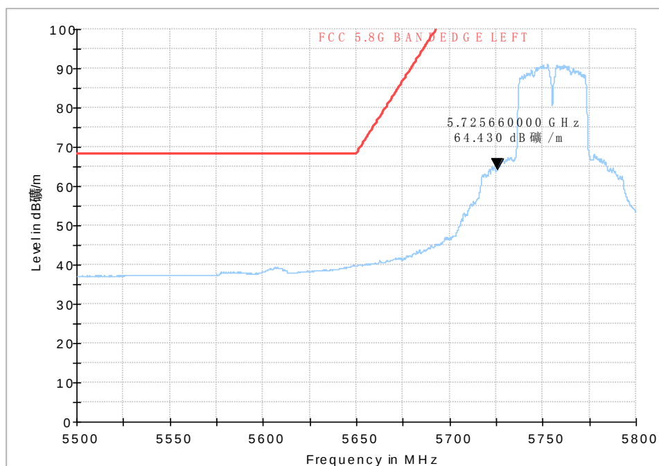
Fig. 53 Band Edges (802.11n-HT40, 5755MHz)
