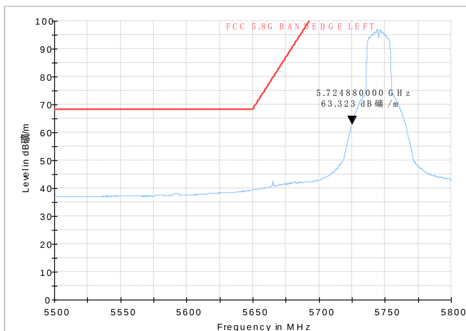
Fig. 49 Band Edges (802.11n-HT20, 5745MHz)
