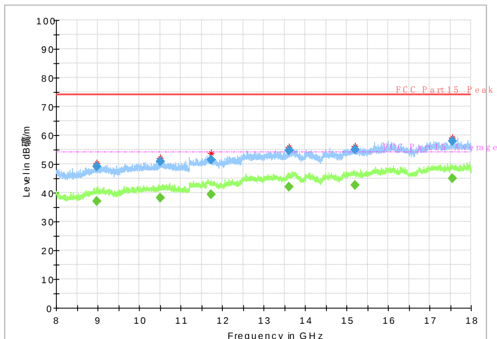
Fig. 38 Radiated Spurious Emission (802.11n-HT40, Ch151, 8 GHz-18 GHz)
