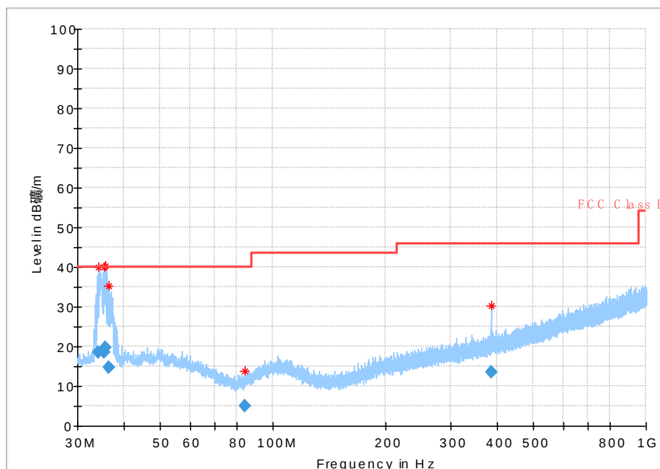
Fig. 42 Radiated Spurious Emission (802.11n-HT40, Ch151, 30 MHz-1 GHz)
