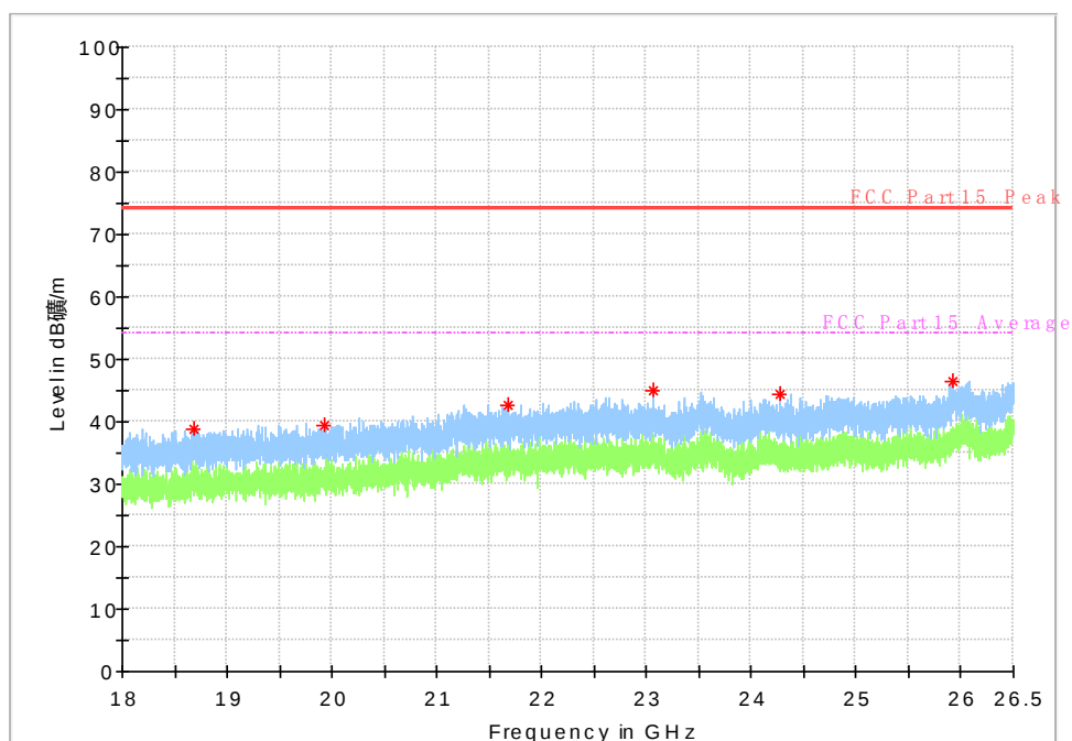
Fig. 45 Radiated Spurious Emission (802.11n-HT40, Ch151 18 GHz-26.5 GHz)
