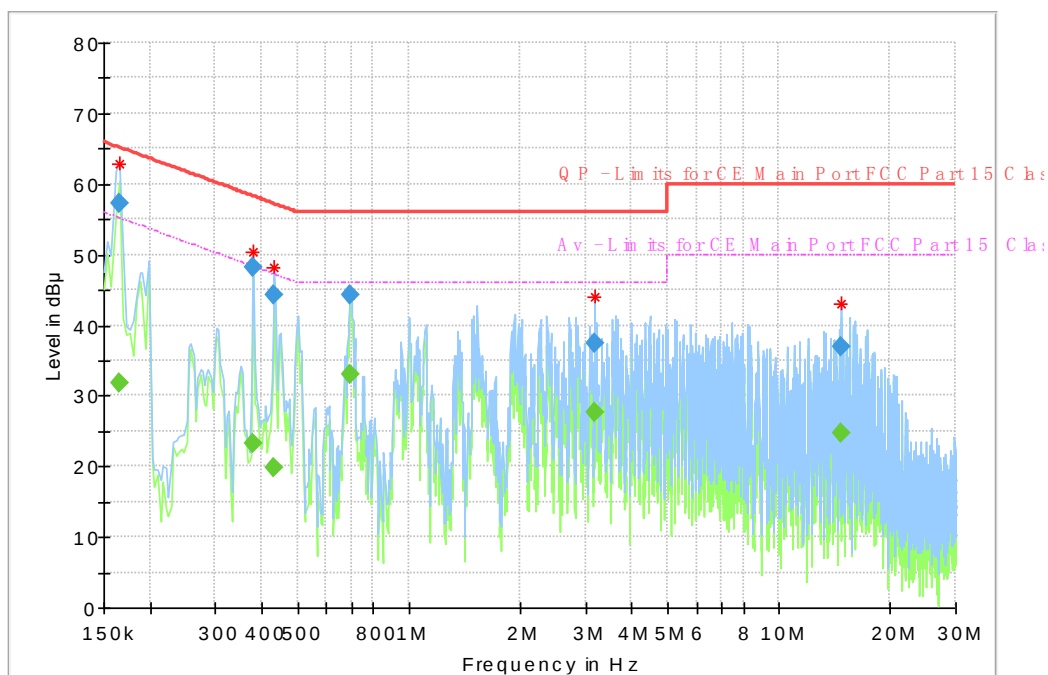
Fig. 55 AC Powerline Conducted Emission-802.11a
