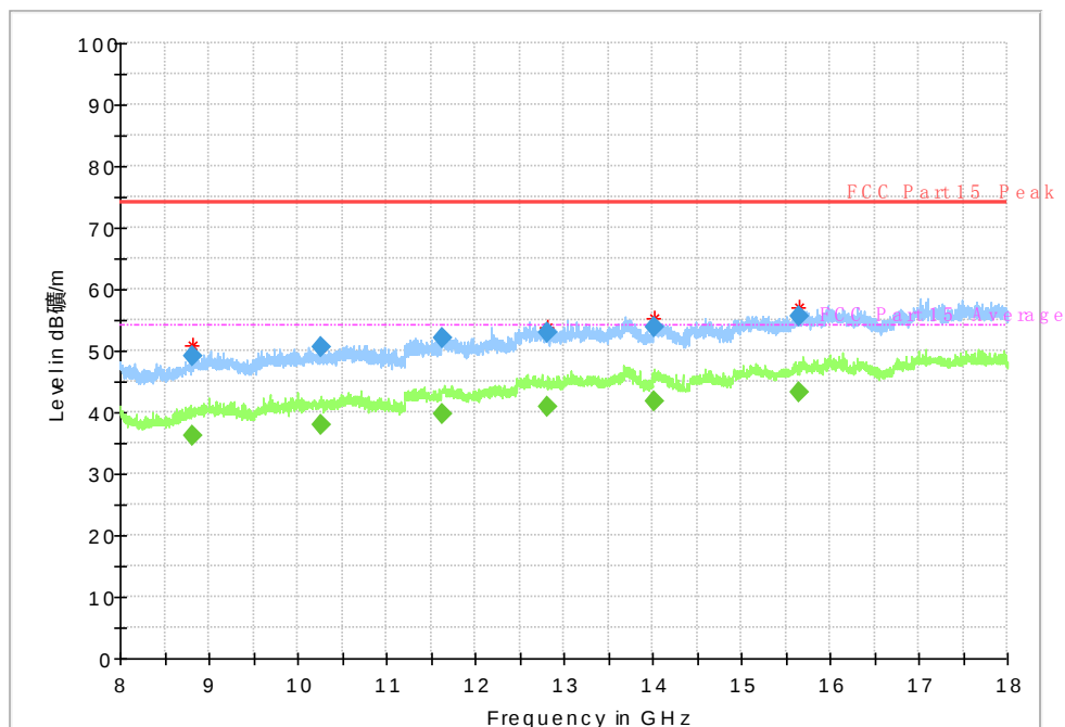
Fig. 28 Radiated Spurious Emission (802.11a, Ch149, 8 GHz-18 GHz)
