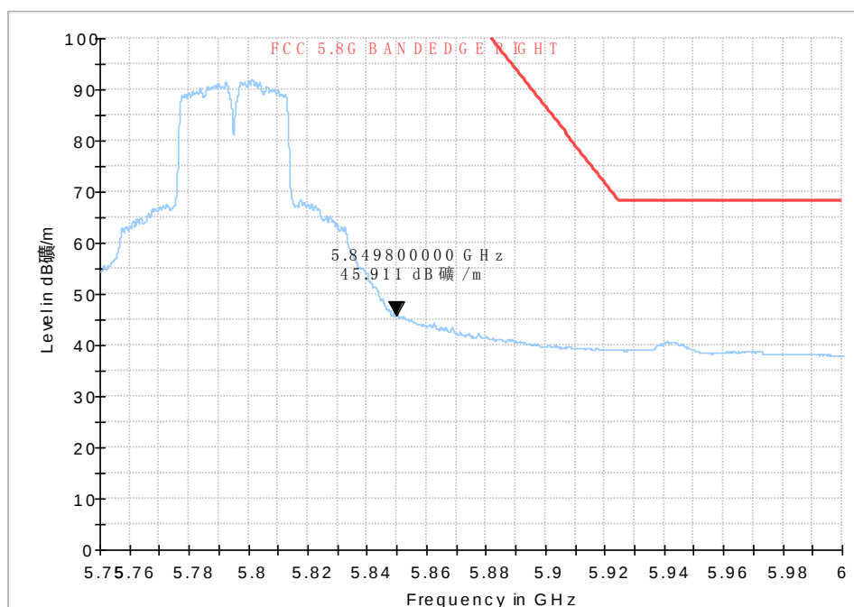
Fig. 54 Band Edges (802.11n-HT40, 5795MHz)
