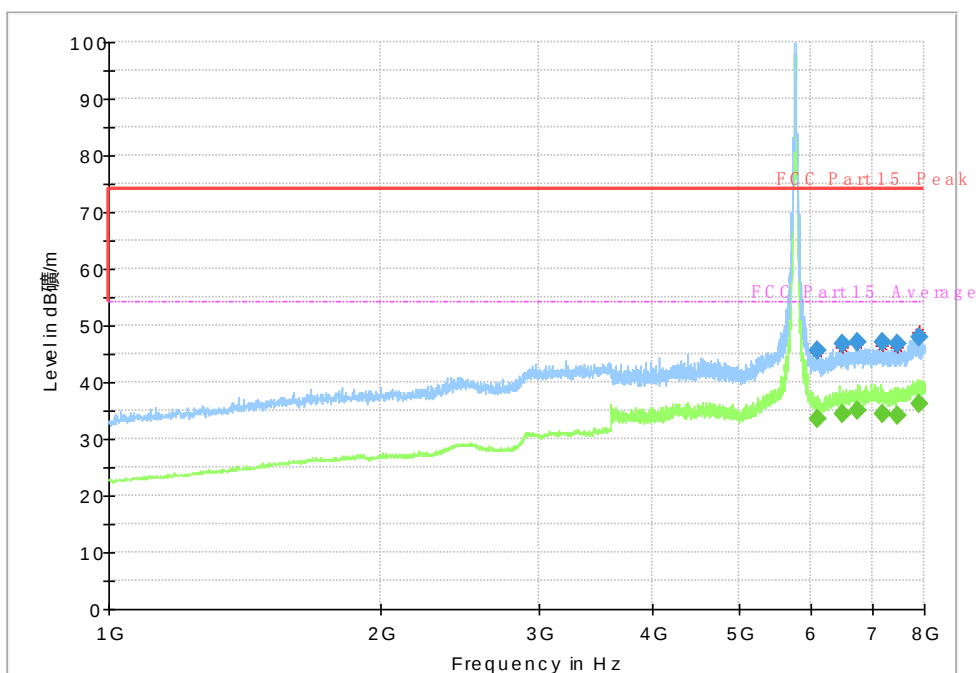
Fig. 43 Radiated Spurious Emission (802.11n-HT40, Ch151, 1 GHz-8 GHz)
