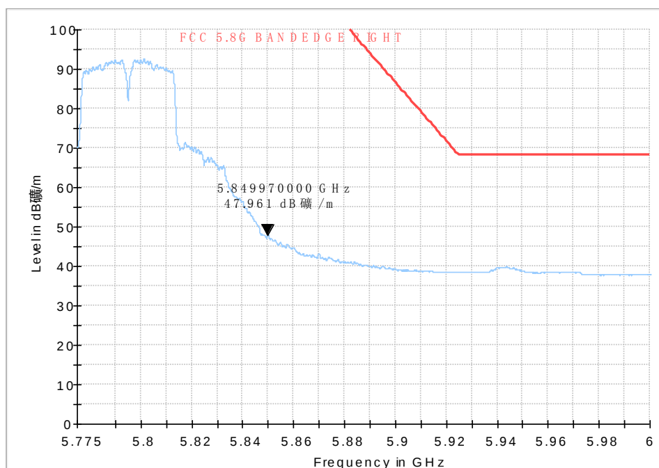
Fig. 52 Band Edges (802.11n-HT40, 5795MHz)
