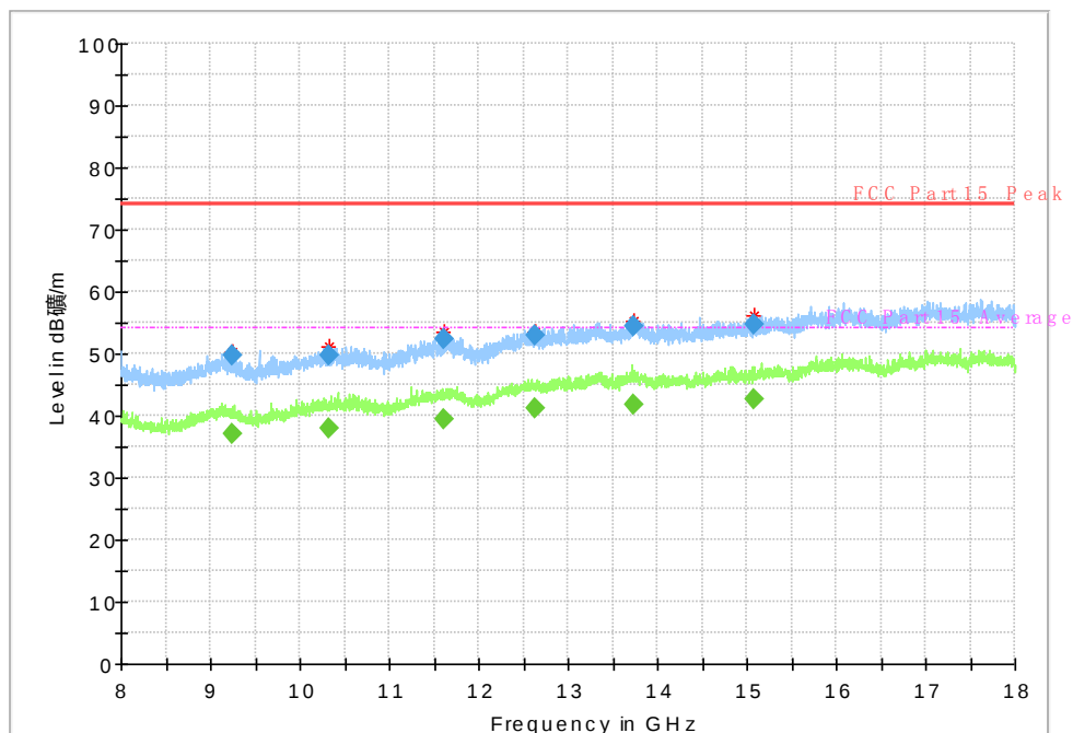
Fig. 44 Radiated Spurious Emission (802.11n-HT40, Ch151, 8 GHz-18 GHz)
