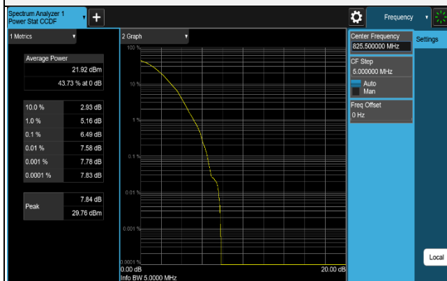
64QAM CH 26805 (825.5MHz)
