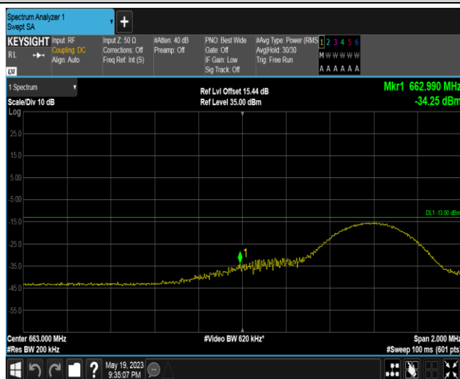
Band71-10MHz-16QAM-133172-1RB#49
