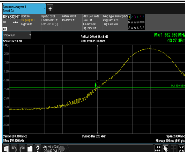
Band71-10MHz-16QAM-133172-1RB#49
