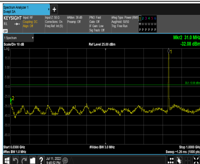
Band26-1.4MHz-16QAM-26915-1RB#0-Range2:30~1000MHz
