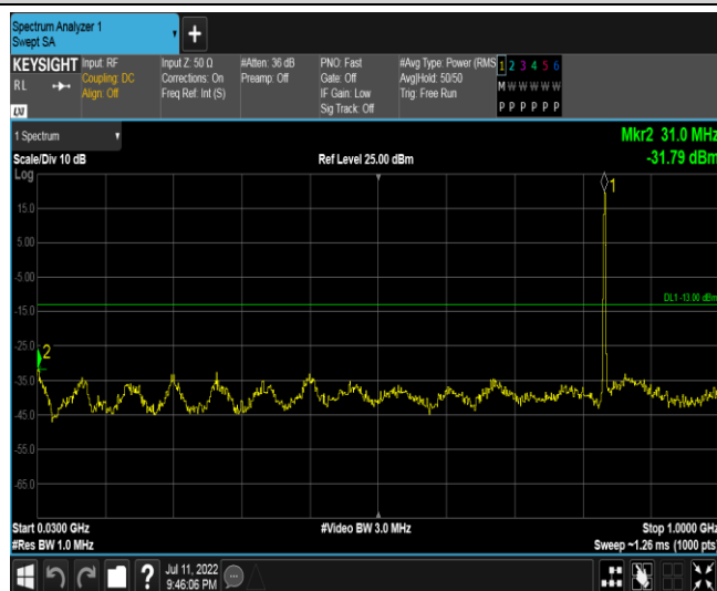
Band26-1.4MHz-16QAM-26915-1RB#0-Range2:30~1000MHz
