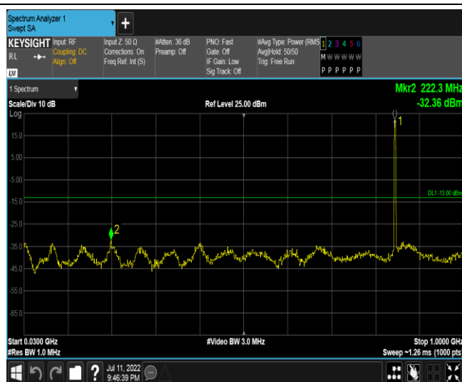
Band26-1.4MHz-QPSK-27033-1RB#0-Range2:30~1000MHz
