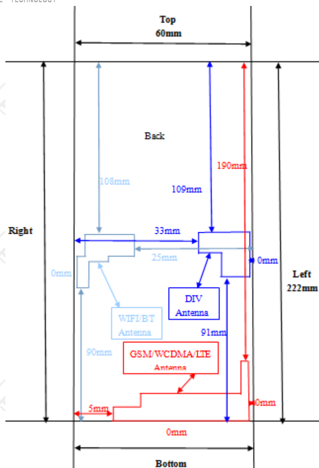
Antenna Configuration 2- open
