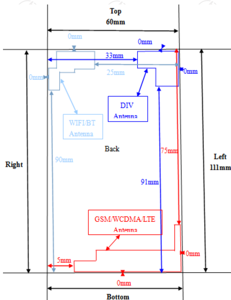
Antenna Configuration 1- close
