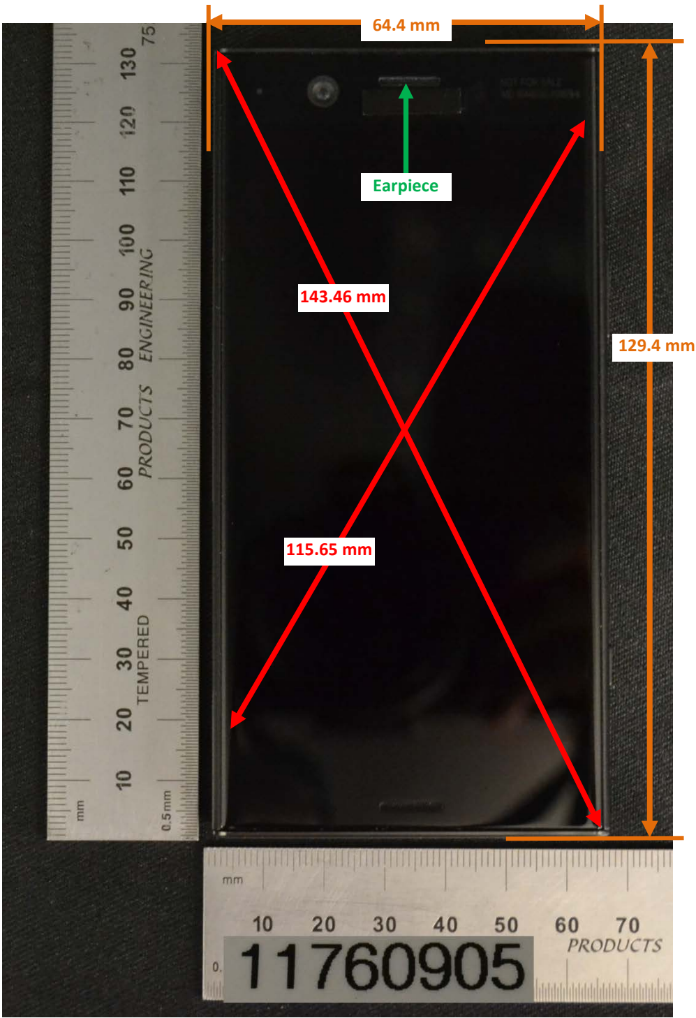
Overall Dimensions
