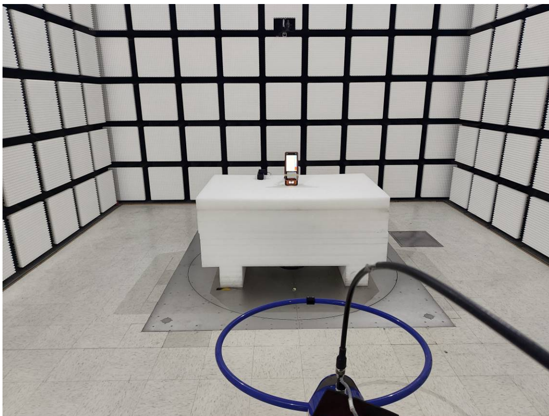
Radiated Emission 9k-30MHz View Ground-parallel
