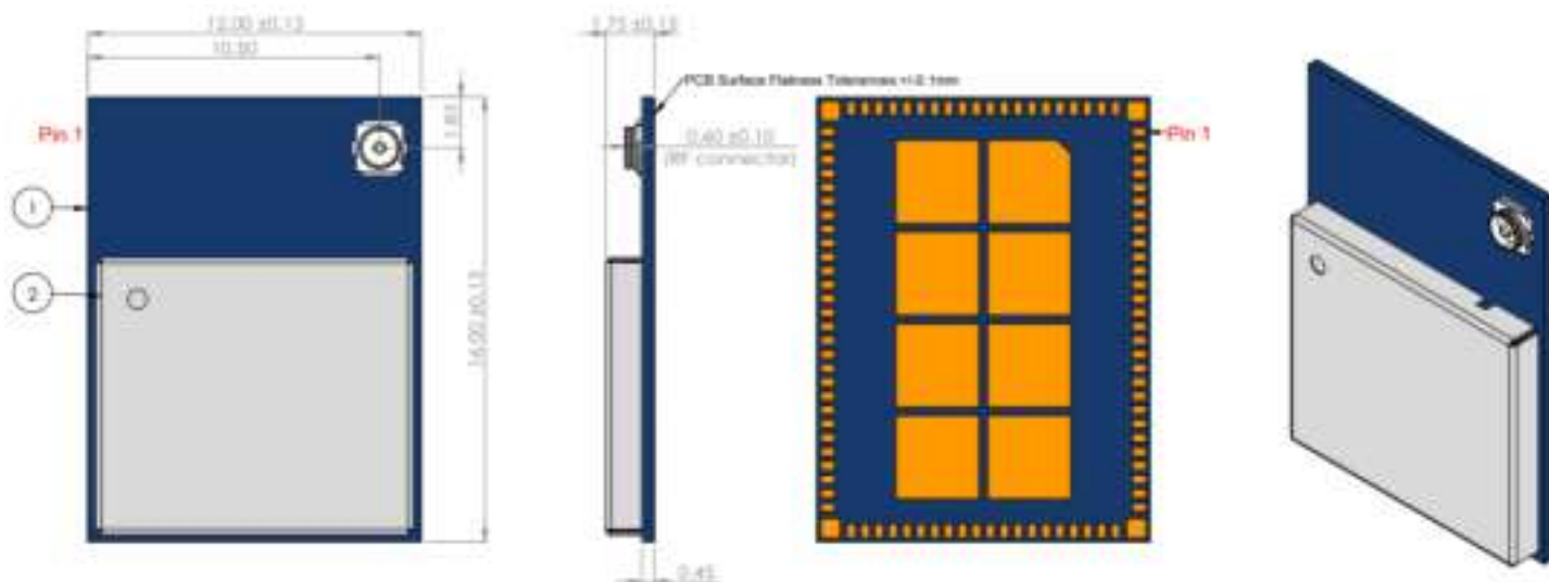
Figure 5: 453-00199 Mechanical Drawing
