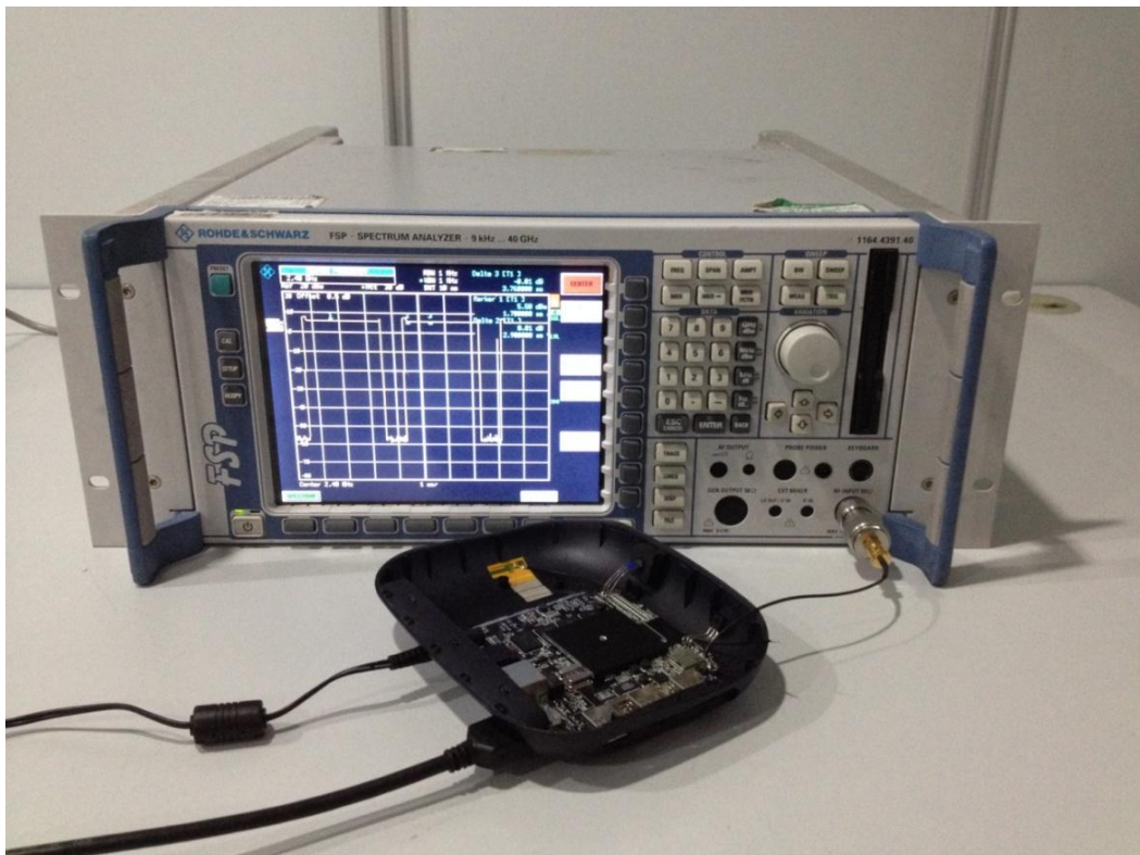
Conducted Test setup photo
