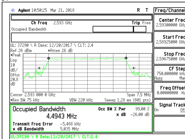
LTE B41 5MHz QPSK Mid Channel RB25-0
