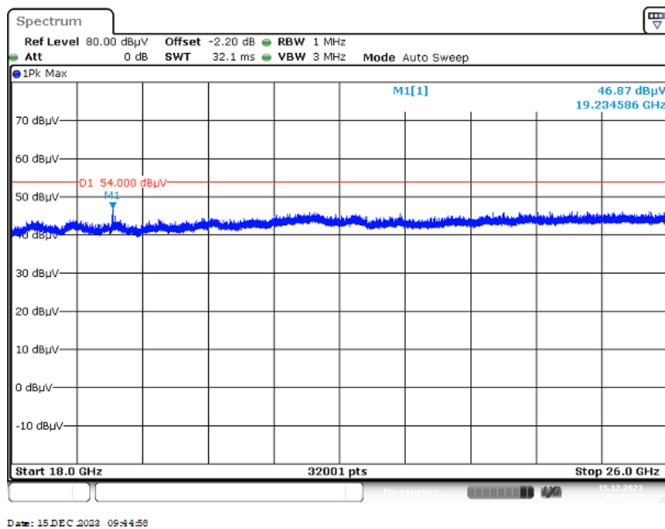
Plot 6: 18 GHz to 26 GHz, TX mode, vertical & horizontal polarization, valid for all channels
