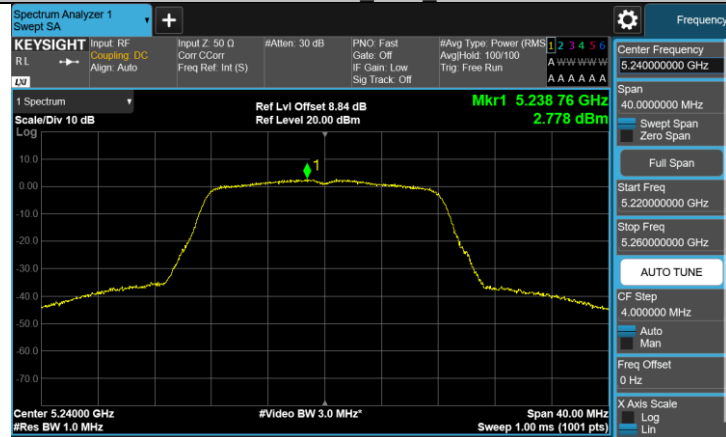
11A-SISO Ant2 5240
