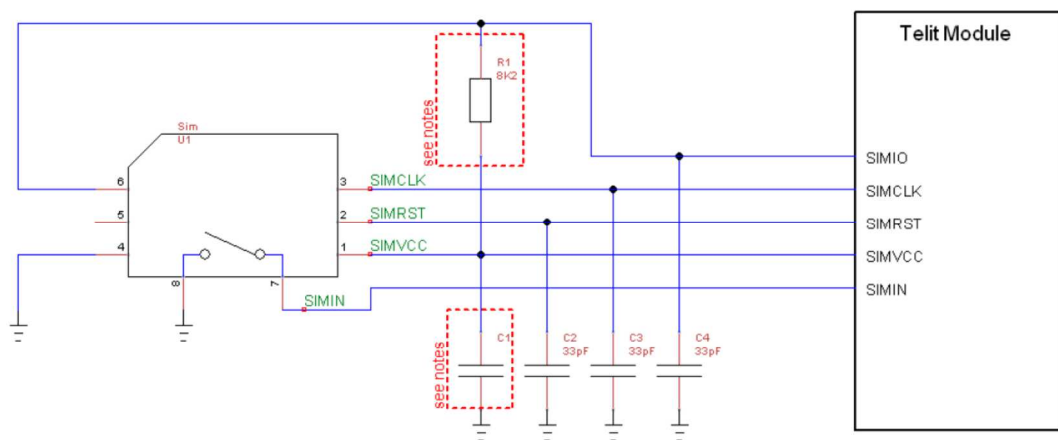
Figure 27: SIM Schematics
