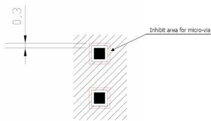
Figure 25: Inhibit Area for Micro-via
