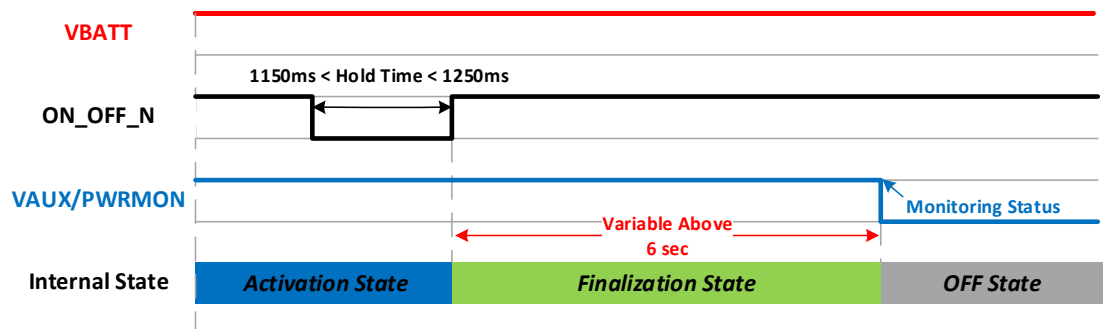
Figure 8: Hardware Shutdown
