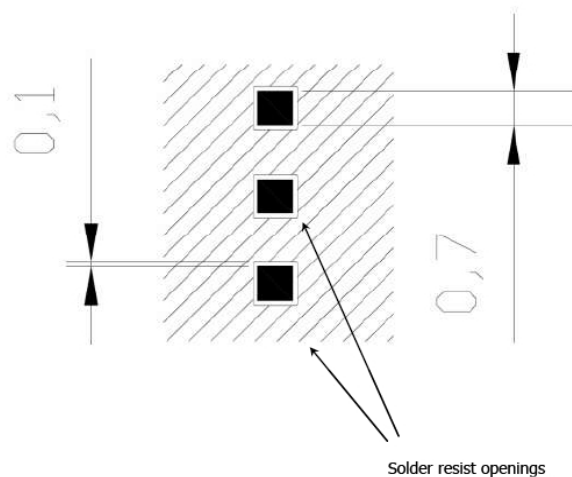
Figure 24: PCB Pad Dimensions
