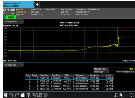
N7(25M)_DFT-s- OFDM_BPSK_Outer_Full_Low_CH
