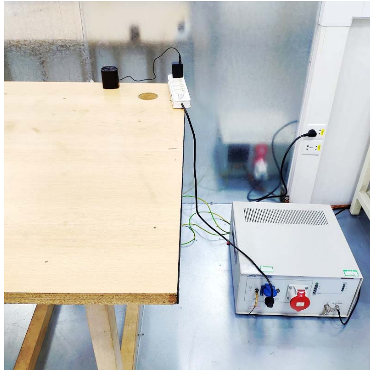
Conducted Emission Test Setup:
