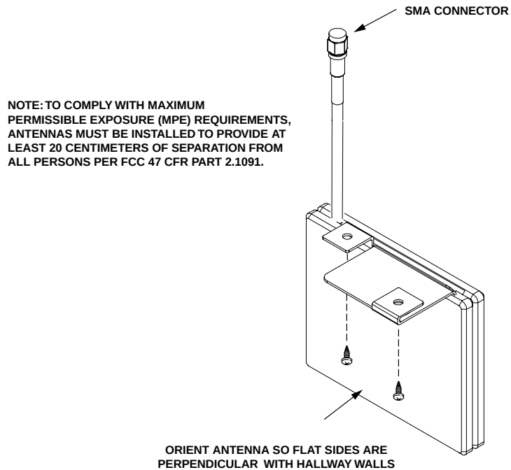
Figure 10. 1900 MHz Ceiling-Mount Hallway Antenna Installation
