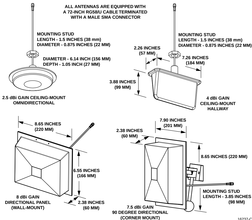
Figure 3. 800 MHz DRU Antenna Options
