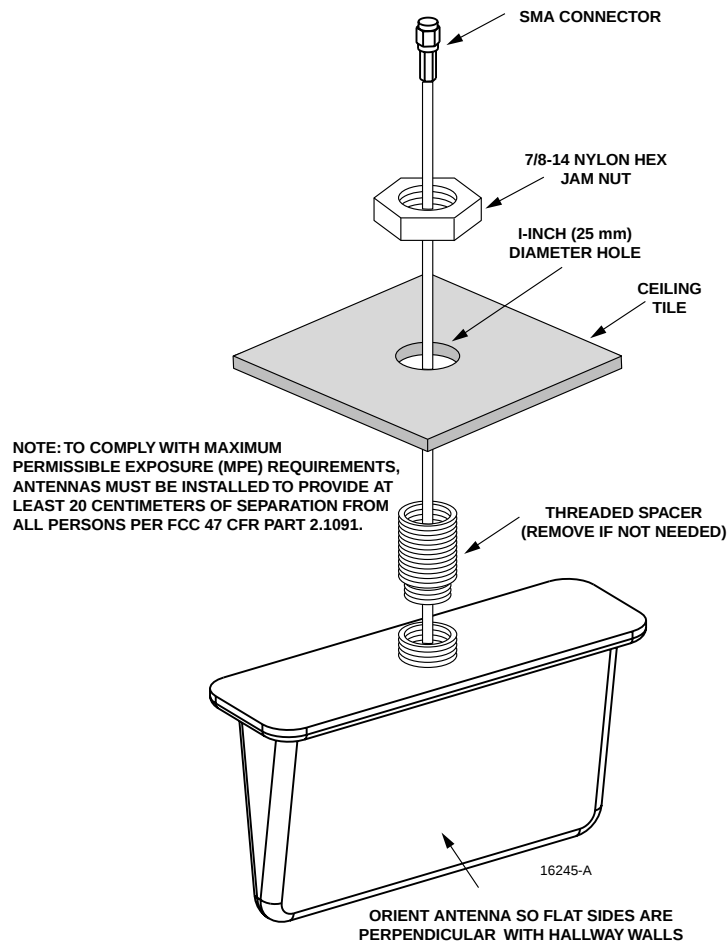
Figure 9. 800 MHz Ceiling-Mount Hallway Antenna Installation
