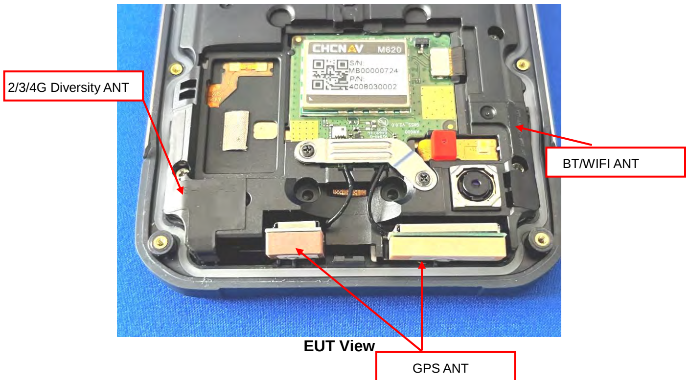
EUT View
