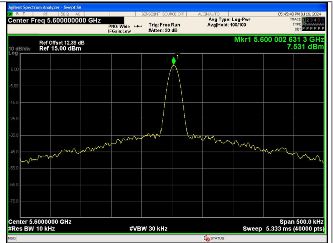
NT/NV_Antenna 0 IEEE 802.11a_Channel 120_20MHz
