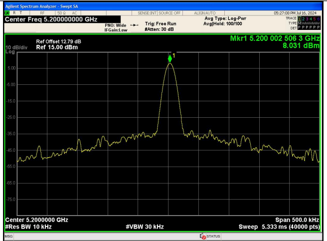
NT/NV_Antenna 0 IEEE 802.11a_Channel 40_20MHz
