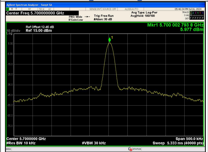
NT/NV_Antenna 0 IEEE 802.11a_Channel 140_20MHz
