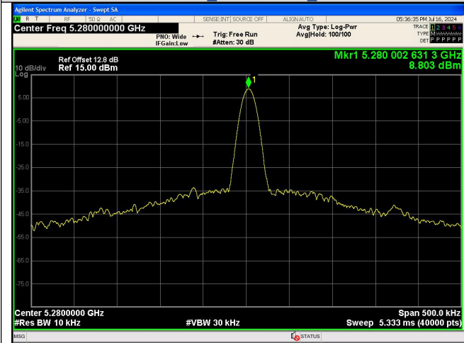
NT/NV_Antenna 0 IEEE 802.11a_Channel 56_20MHz
