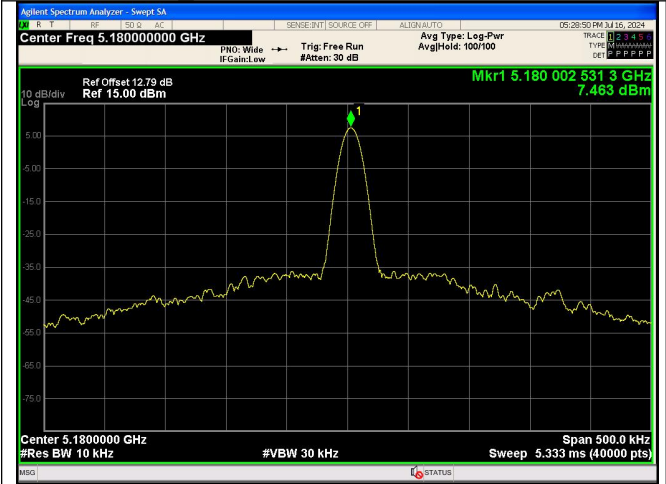
NT/NV_Antenna 0 IEEE 802.11n_Channel 36_20MHz
