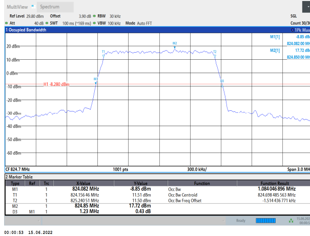
Band5-1.4MHz-QPSK-20525-6RB#0
