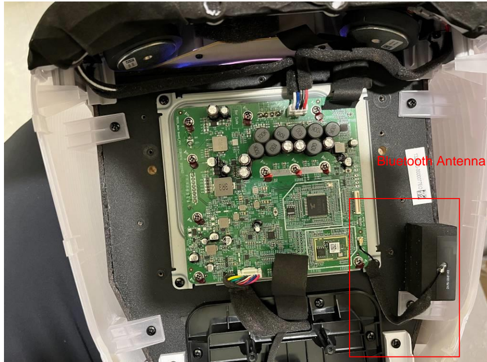
Figure 1. Internal view
