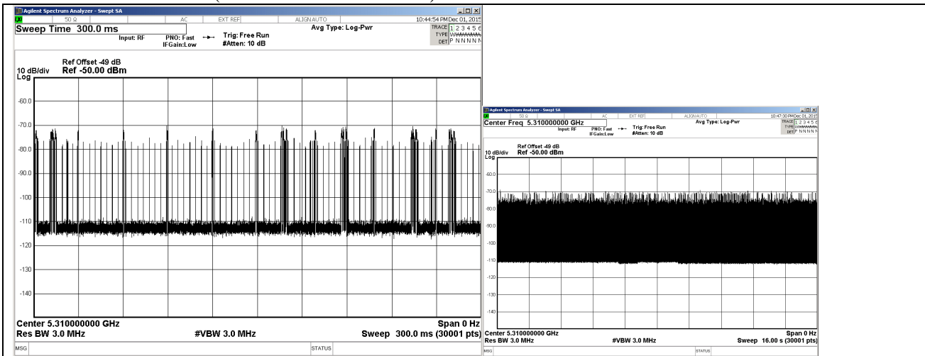
Plots of WLAN Traffic (traffic was about 17 % over)
