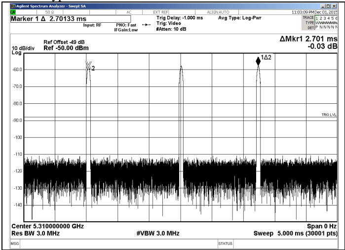
Plots of WLAN Traffic (traffic was about 17 % over)
