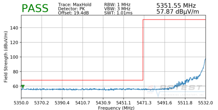
Plot 7-111. Radiated Lower Band Edge Plot (Peak – UNII Band 2C-Interior)
