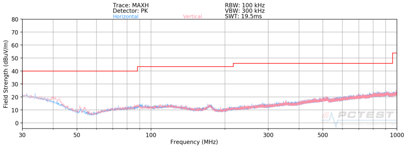
Plot 7-123. Radiated Spurious Plot below 1GHz (802.11a – U3 Ch. 157)
