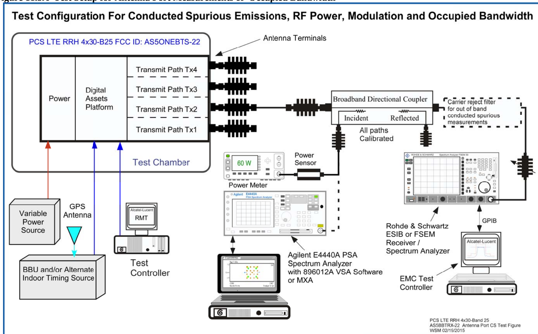
Figure 11.5A Test Setup for Antenna Port Measurements of Occupied Bandwidth
