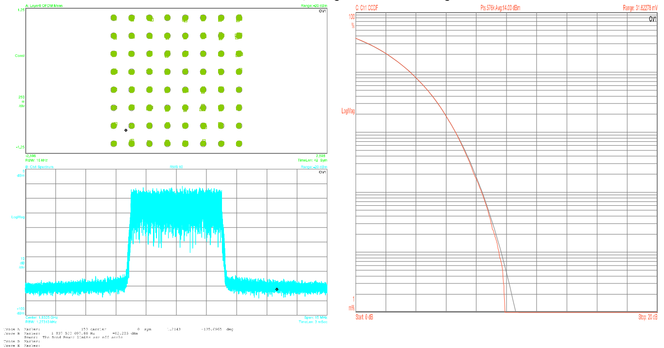
FIGURE 13D CODE DOMAIN A BLOCK, 64QAM 5 MHz 64QAM & PAR= 10dB
