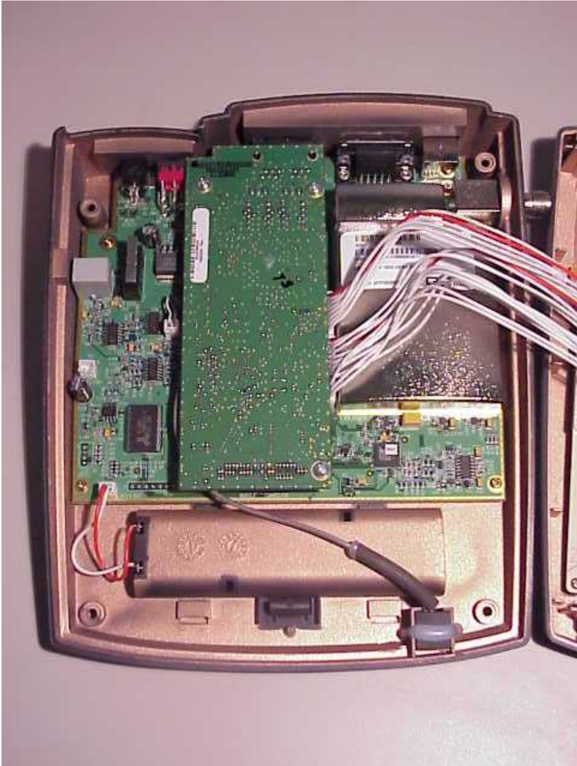
Figure 3: Bottom cover wit circuit boards installed – SX5D
