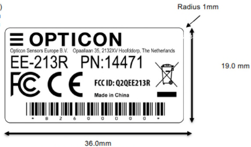
Figure 3: Product Label dimensions
