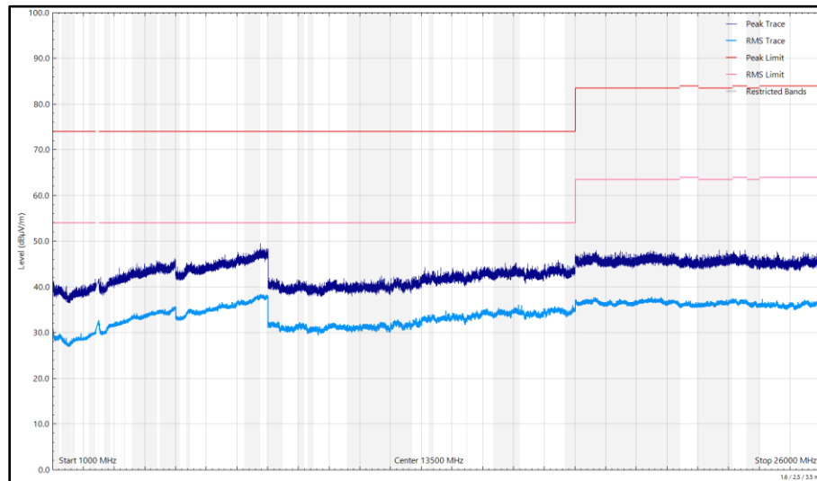
Figure 56 - 2475 MHz (CH25), Thread, ePA, Core 0, 1 GHz to 26 GHz, Horizontal
