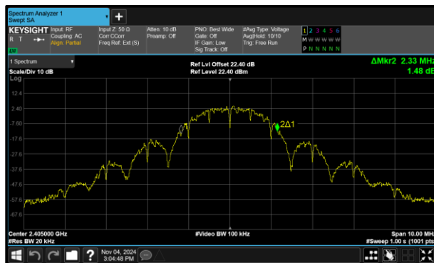
Figure 21 - Core 1 (B) 2405 MHz (CH11) 99% Bandwidth
