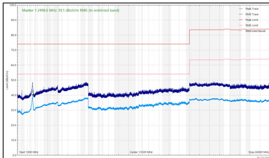
Figure 57 - 2475 MHz (CH25), Thread, ePA, Core 0, 1 GHz to 26 GHz, Vertical
