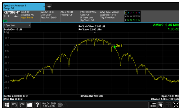
Figure 15 - Core 0 (A) 2405 MHz (CH11) 99% Bandwidth
