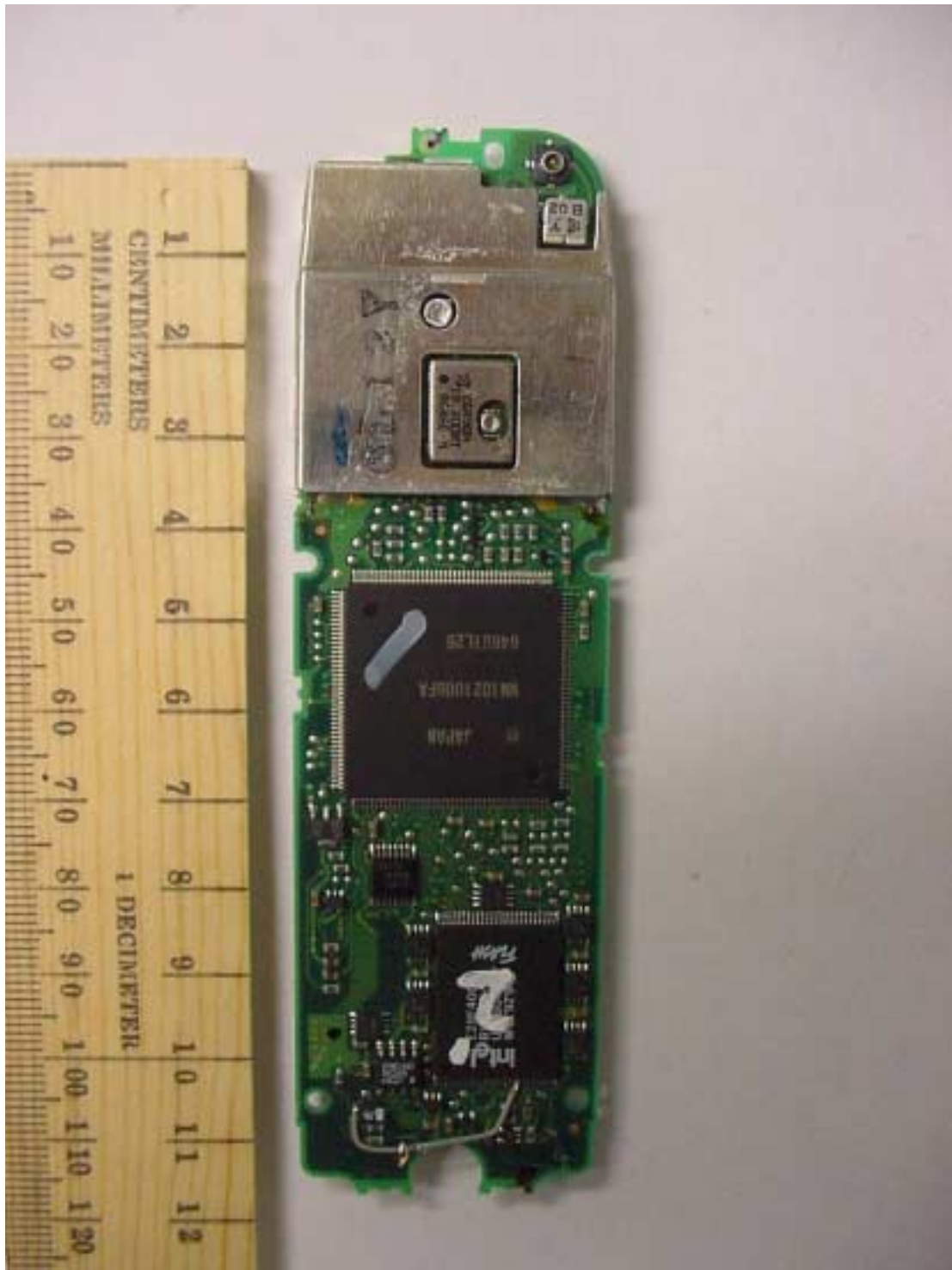
PHOTOGRAPH 8: TOP OF RF PCB WITH SHIELDS
