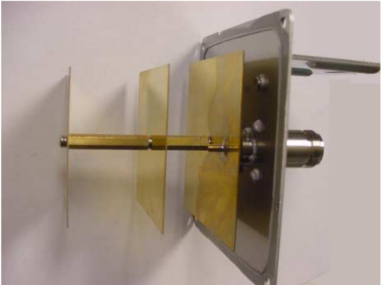
PHOTOGRAPH 15: INSIDE OF ANTENNA
