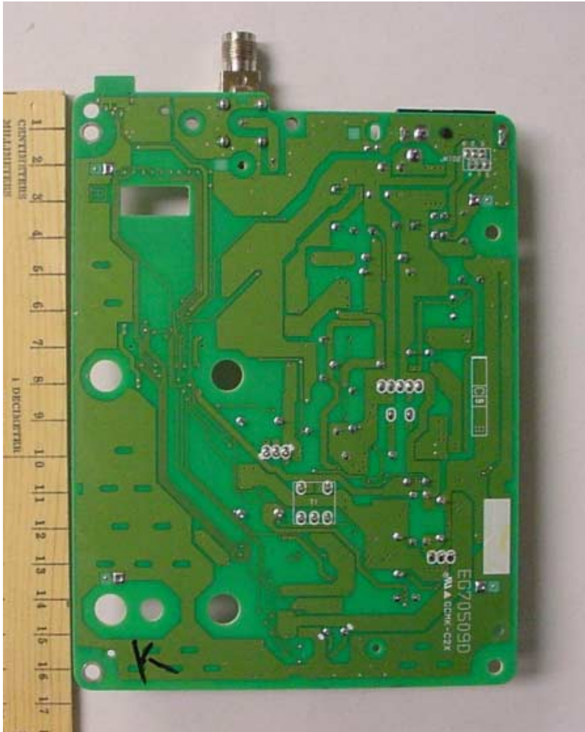
PHOTOGRAPH 6: BOTTOM OF MAIN PCB
