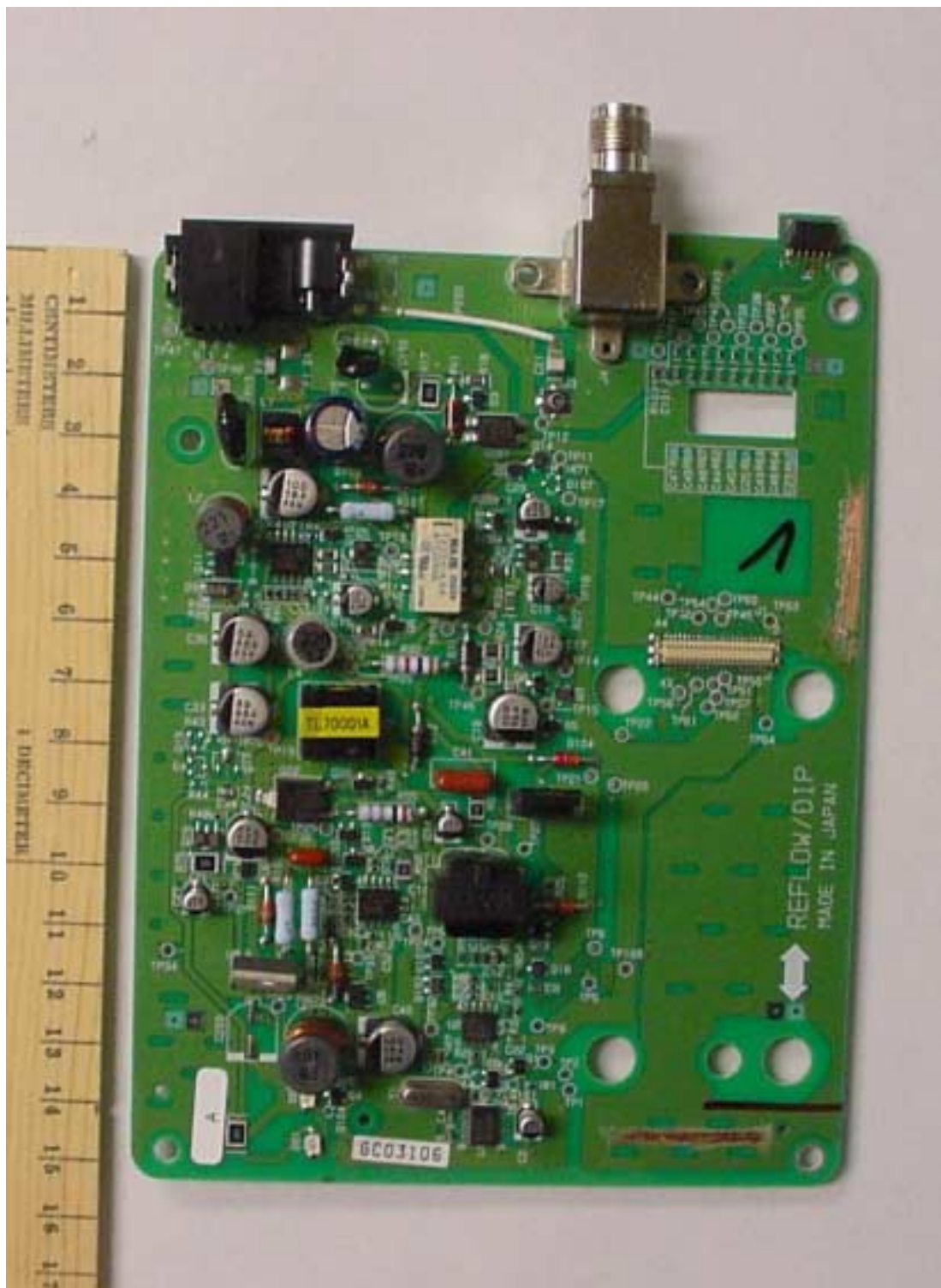
PHOTOGRAPH 7: TOP OF MAIN PCB
