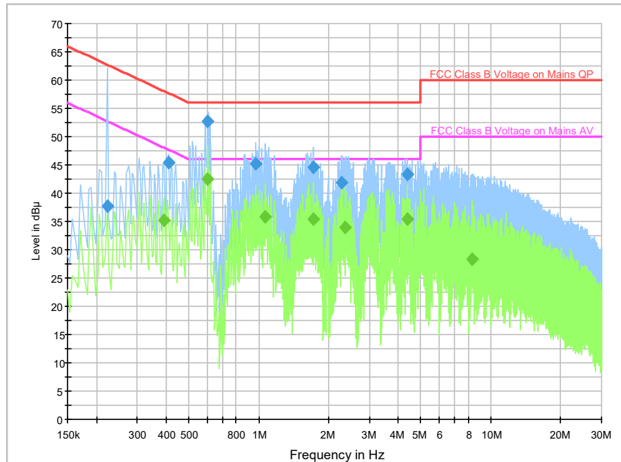
Fig.67 Conducted Emission (802.11a, Ch36, TX)
