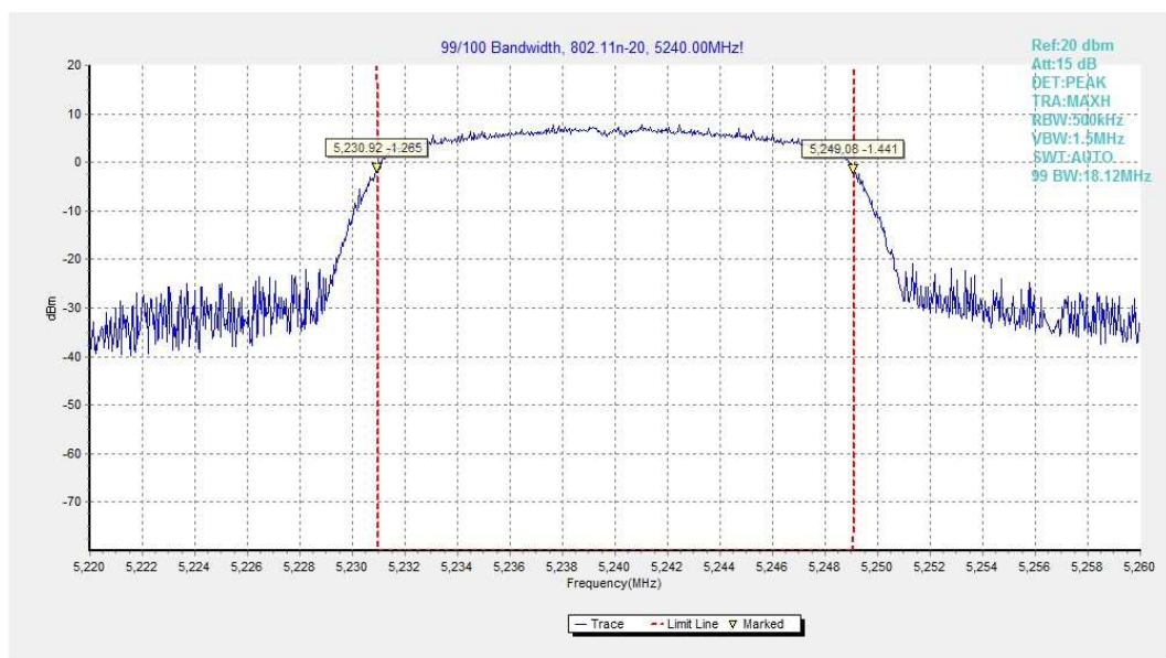
Fig.74 99% Occupied bandwidth (802.11n-HT20, 5240MHz)
