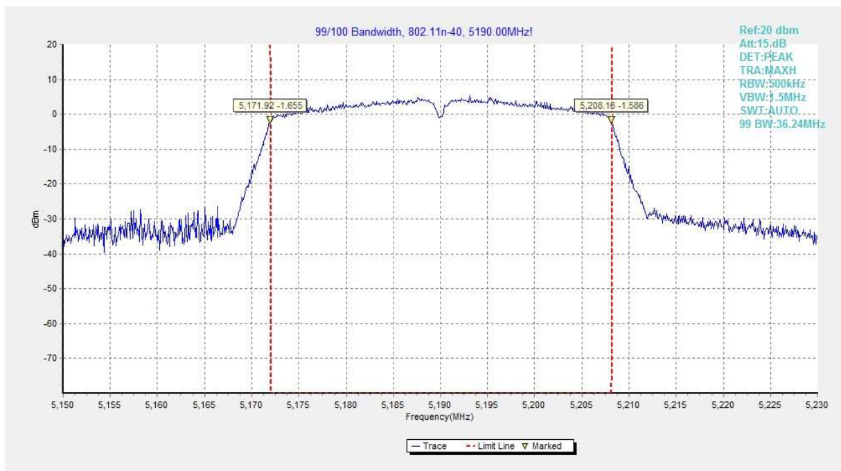
Fig.75 99% Occupied bandwidth (802.11n-HT40, 5190MHz)
