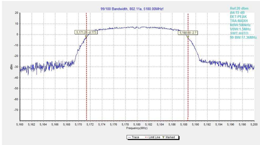
Fig.69 99% Occupied bandwidth (802.11a, 5180MHz)
