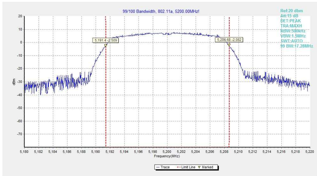
Fig.70 99% Occupied bandwidth (802.11a, 5200MHz)
