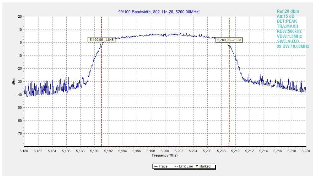
Fig.73 99% Occupied bandwidth (802.11n-HT20, 5200MHz)
