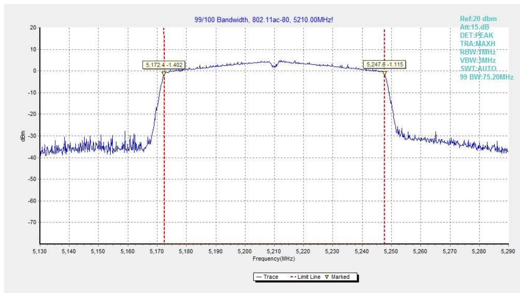
Fig.77 99% Occupied bandwidth (802.11ac-HT80, 5210MHz)
