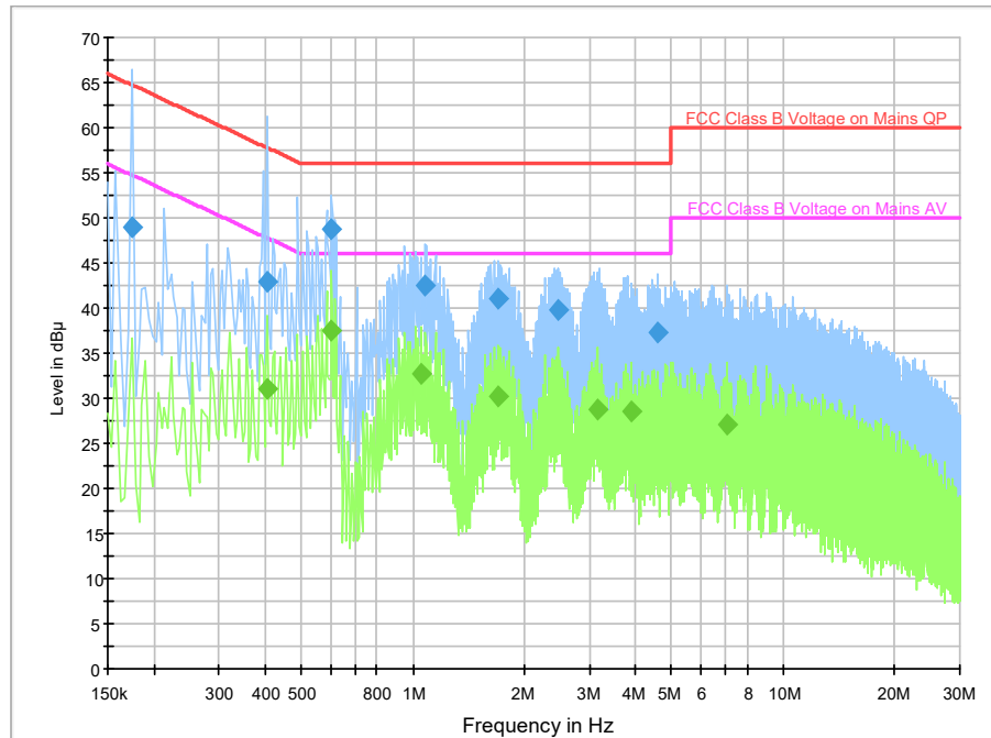
Fig.68 Conducted Emission(802.11a, IDLE)
