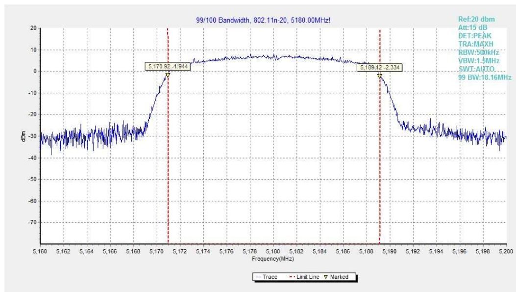
Fig.72 99% Occupied bandwidth (802.11n-HT20, 5180MHz)
