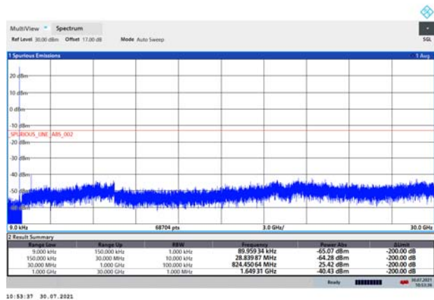
LTE eMTC Band 26 3MHz CH-Middle 9kHz~30GHz
