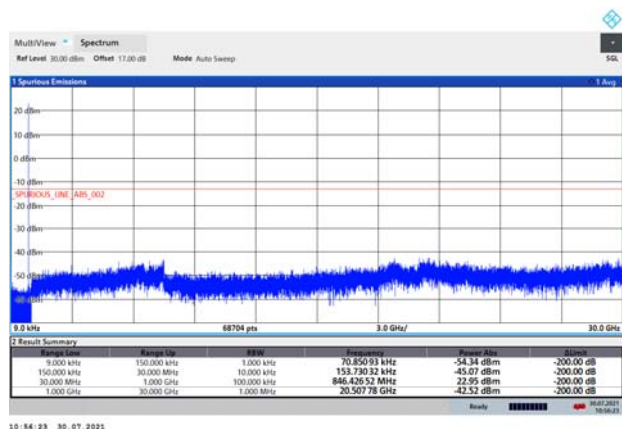
LTE eMTC Band 26 3MHz CH-High 9kHz~30GHz
